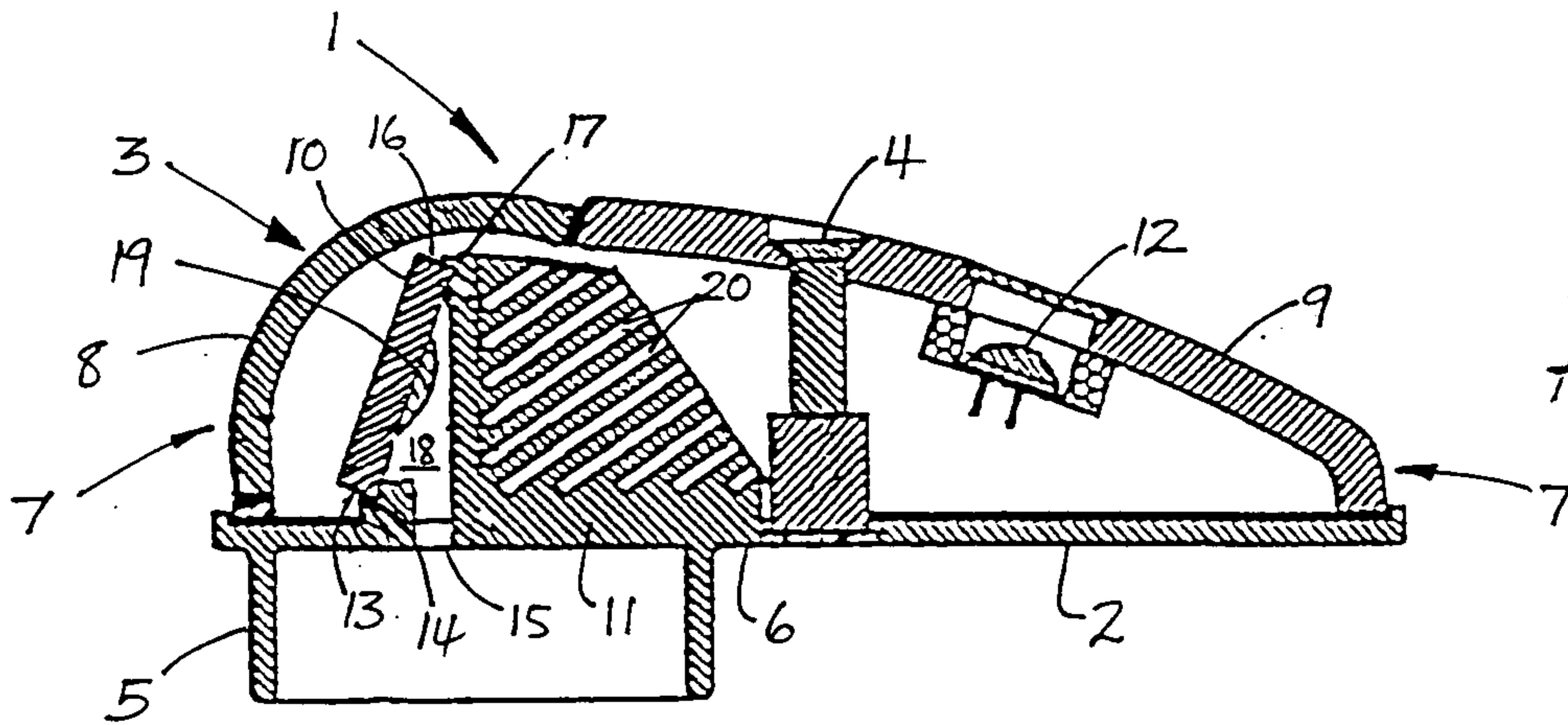
SECTION X-X
