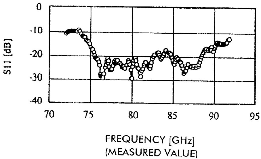
RETURN LOSS
