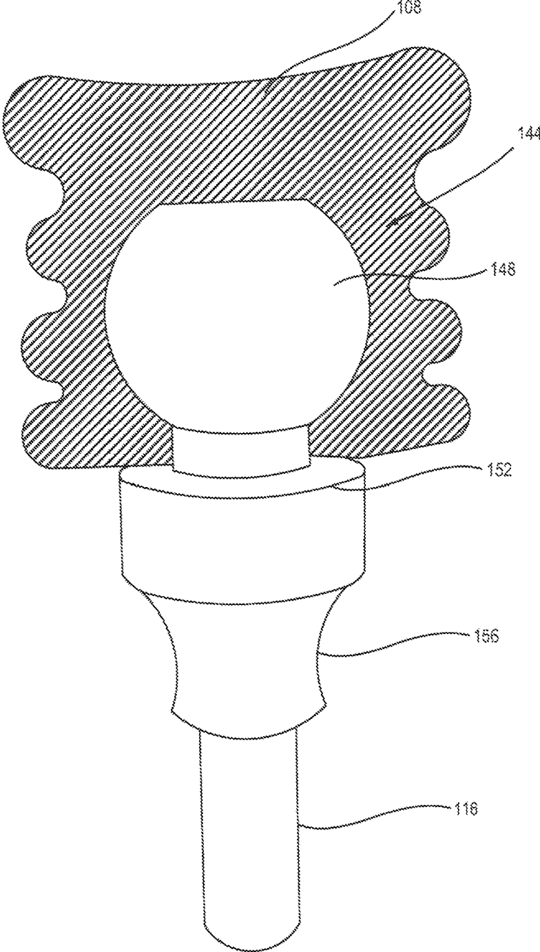
FIG. 7 PRIOR ART
