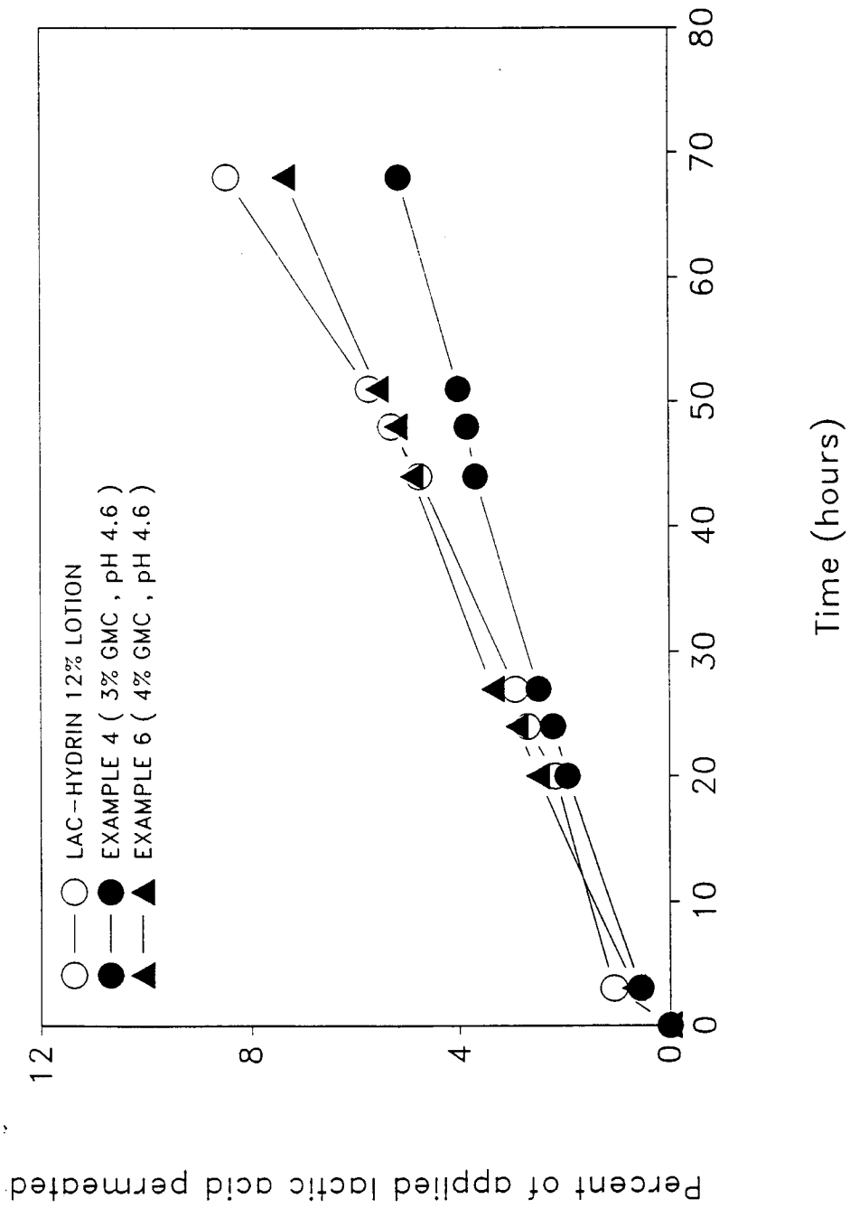
FIGURE 5 SKIN PERMEATION OF LACTIC ACID FROM LYSINE LACTATE 12% LOTIONS AND LAC-HYDRIN 12% LOTION
