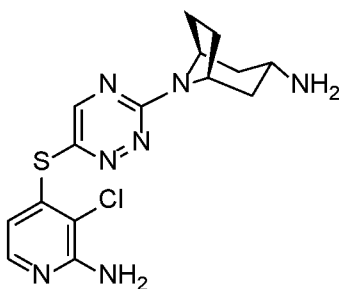
(1 R ,3 s ,5 S )-8-((2-amino-3-chloropyridin-4-yl)thio)-1,2,4-triazin-3-yl)-8-azabicyclo[3.2.1]octan-3-amine
