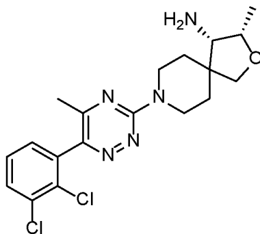
(3 S ,4 S )-8-(6-(2,3-dichlorophenyl)-5-methyl-1,2,4-triazin-3-yl)-3-methyl-2-oxa-8-azaspiro[4.5]decan-4-amine
