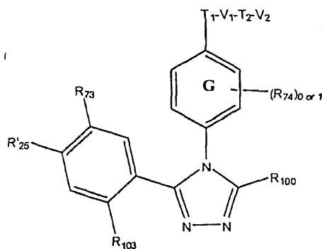
(XXXIX) and
