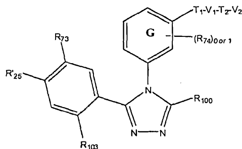
(XL)
