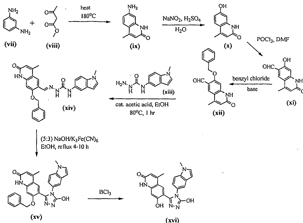
Scheme VII: Alternative synthesis of triazole compounds of the invention
