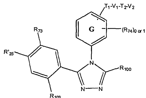
(XXXVIII)
