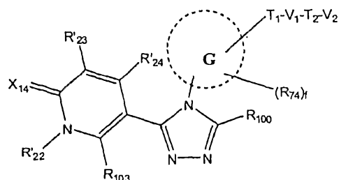
(XXX)
