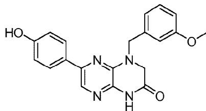
6-(4-hydroxyphenyl)-4-(3-methoxybenzyl)-3,4-dihydropyrazino[2,3-b]pyrazin-2(1H)-one;
