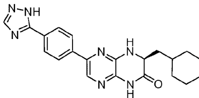
(R)-6-(4-(1H-1,2,4-triazol-5-yl)phenyl)-3-(cyclohexylmethyl)-3,4-dihydropyrazino[2,3-b]pyrazin-2(1H)-one.
