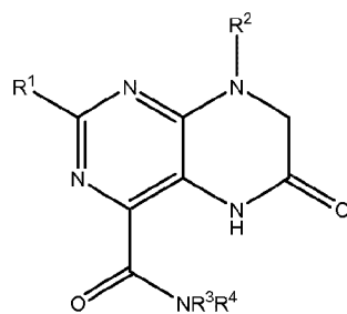
(IIc)
