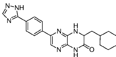
6-(4-(1H-1,2,4-triazol-5-yl)phenyl)-3-(cyclohexylmethyl)-3,4-dihydropyrazino[2,3-b]pyrazin-2(1H)-one;
