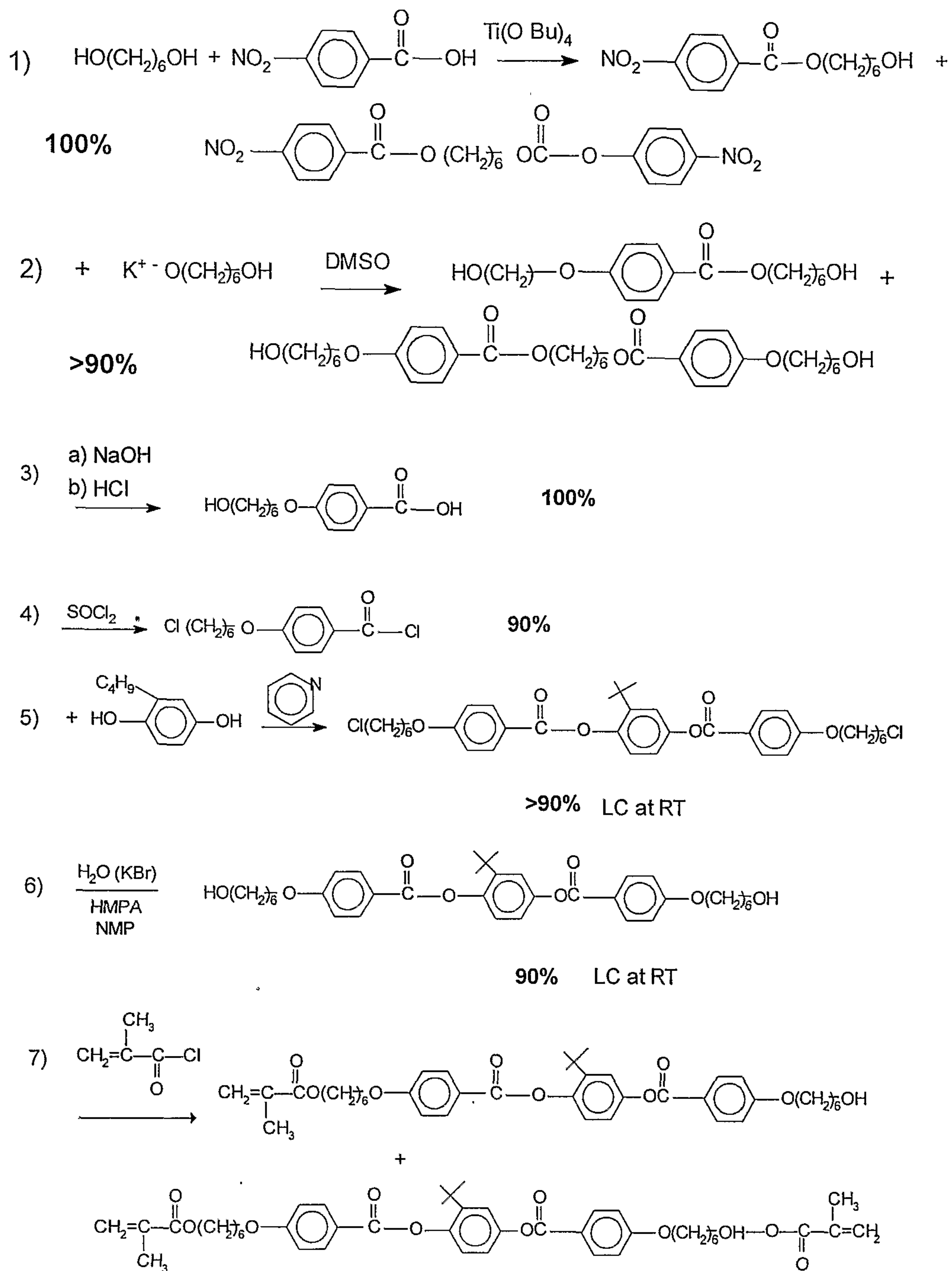
Scheme 2.
