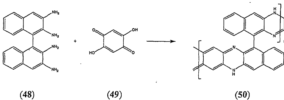
Reaction scheme E
