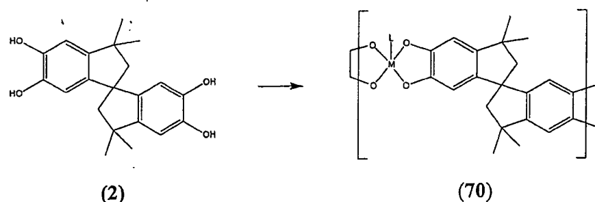
Reaction scheme J
