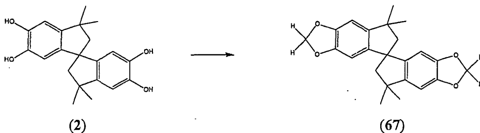
Reaction scheme G
