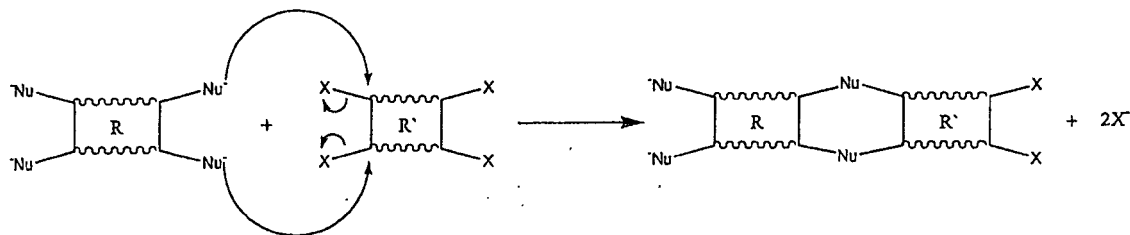
Reaction scheme B
