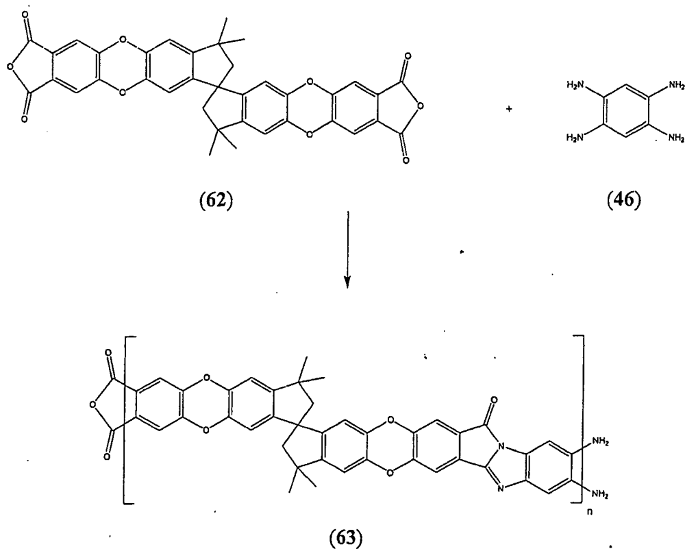
Reaction scheme F
