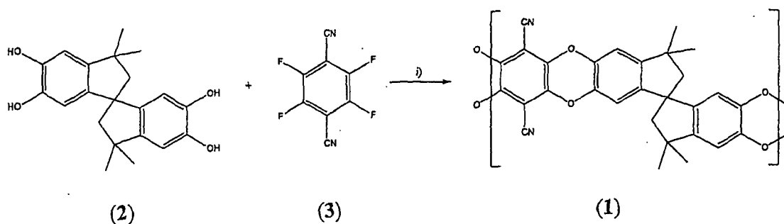
Reaction scheme A: synthesis of polydioxane A (1); i) \text{K}_2\text{CO}_3 , DMF, 50^\circ\text{C}
