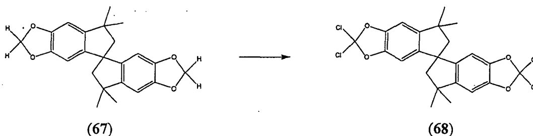
Reaction scheme H
