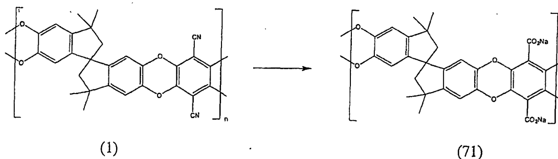
Reaction scheme K
