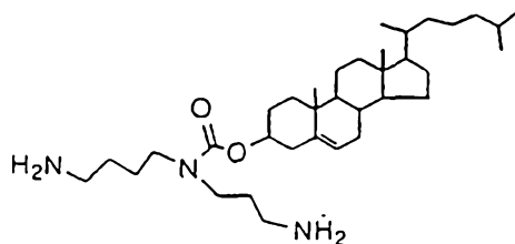
( spermidine cholesterol carbamate )
