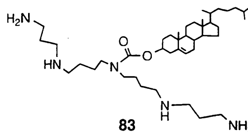
N,N-Bis(N'-3-aminopropyl-N''-4-aminobutyl) cholesteryl carbamate
