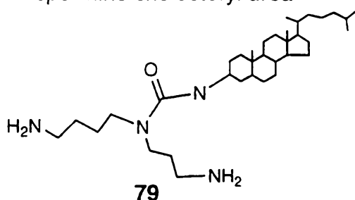
N 4 -spermidine dihydro cholesteryl urea
