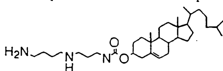
(N 1 -spermidine cholesteryl carbamate).
