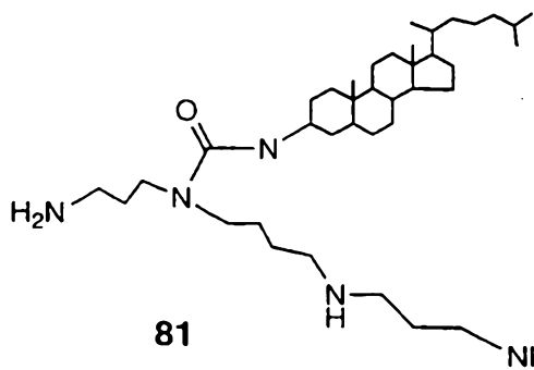
N 4 -spermine dihydro cholesteryl urea
