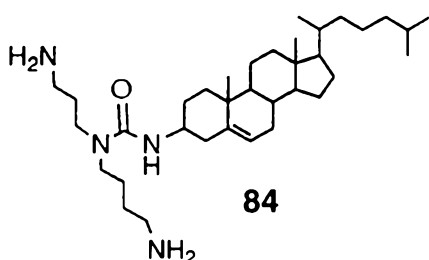
N 4 -spermidine cholesteryl urea
