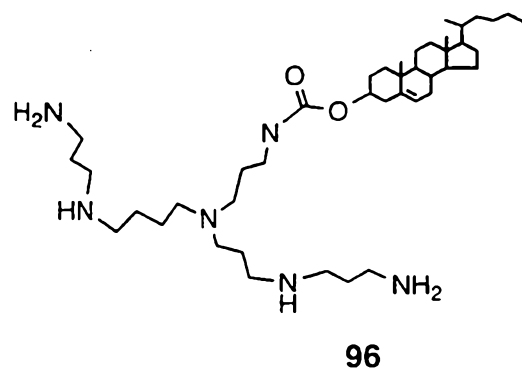
N-[N 1 ,N 4 ,N 8 -Tris(3-aminopropyl) spermidine] cholesteryl carbamate
