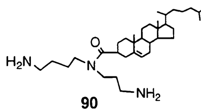
N 4 Spermidine cholesteryl carboxamide
