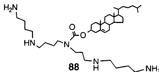
N,N-Bis(N'-3-aminopropyl-N''-4-aminobutyl) cholesteryl carbamate
