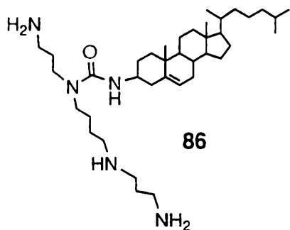
N 4 -spermine cholesteryl urea
