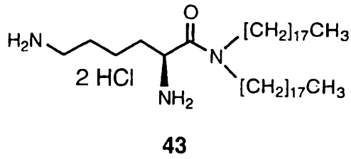
N,N-dioctadecyllysineamide diHCl salt
