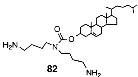
N,N-Bis(4-aminobutyl) cholesteryl carbamate
