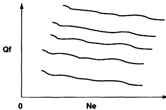
MAP OF PILOT INJECTION QUANTITY LEARNING VALUE
