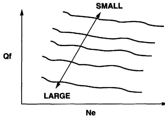
MAP OF PILOT INJECTION RATIO LEARNING VALUE
