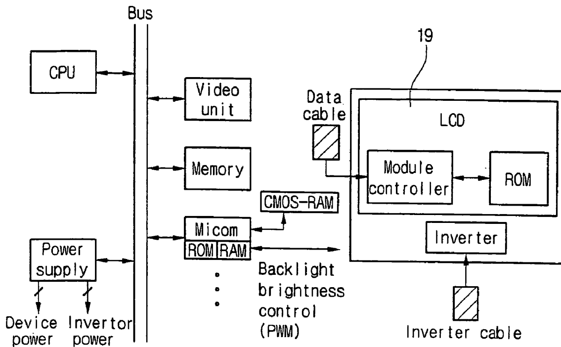
Fig. 1 Related Art
