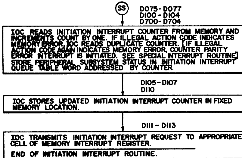
INITIATION INTERRUPT ROUTINE FIG. 187
