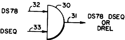
AND-GATE FIG. 3a
