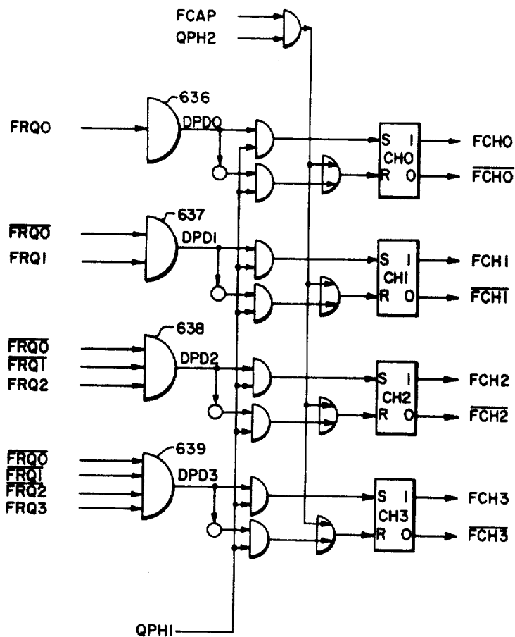
PERIPHERAL CHANNEL SERVICE REQUEST PRIORITY LOGIC
