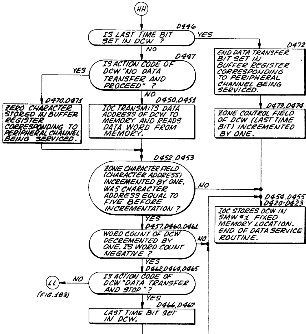
DATA SERVICE ROUTINE FIG. 184 e
