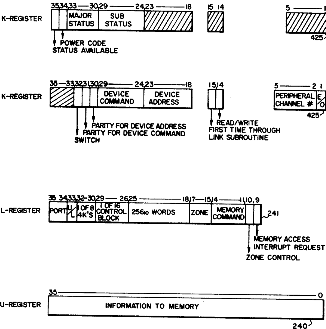
REGISTERS-PROCESSING AND CONTROL UNIT FIG. 34b.
