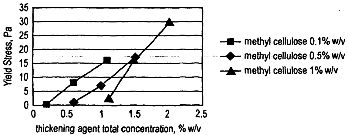
Yield Stress Data at Different Excipient Concentrations
