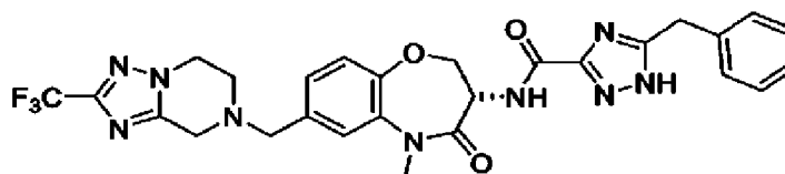
(S)-5-benzyl-N-(5-methyl-4-oxo-7-((2-(trifluoromethyl)-5,6-dihydro-[1,2,4]triazolo[1,5-a]pyrazin-7(8H)-yl)methyl)-2,3,4,5-tetrahydrobenzo[b][1,4]oxazepin-3-yl)-1H-1,2,4-triazole-3-carboxamide
