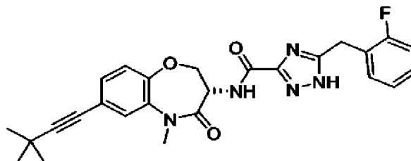
(S)-N-(7-(3,3-dimethylbut-1-yn-1-yl)-5-methyl-4-oxo-2,3,4,5-tetrahydrobenzo[b][1,4]oxazepin-3-yl)-5-(2-fluorobenzyl)-1H-1,2,4-triazole-3-carboxamide
