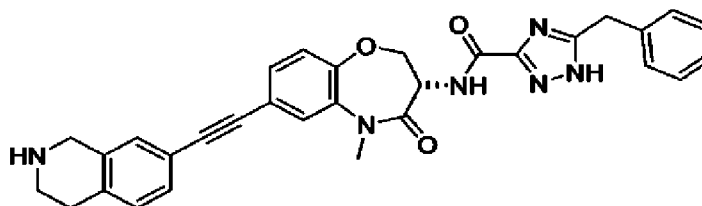
(S)-5-benzyl-N-(5-methyl-4-oxo-7-((1,2,3,4-tetrahydroisoquinolin-7-yl)ethynyl)-2,3,4,5-tetrahydrobenzo[b][1,4]oxazepin-3-yl)-1H-1,2,4-triazole-3-carboxamide
