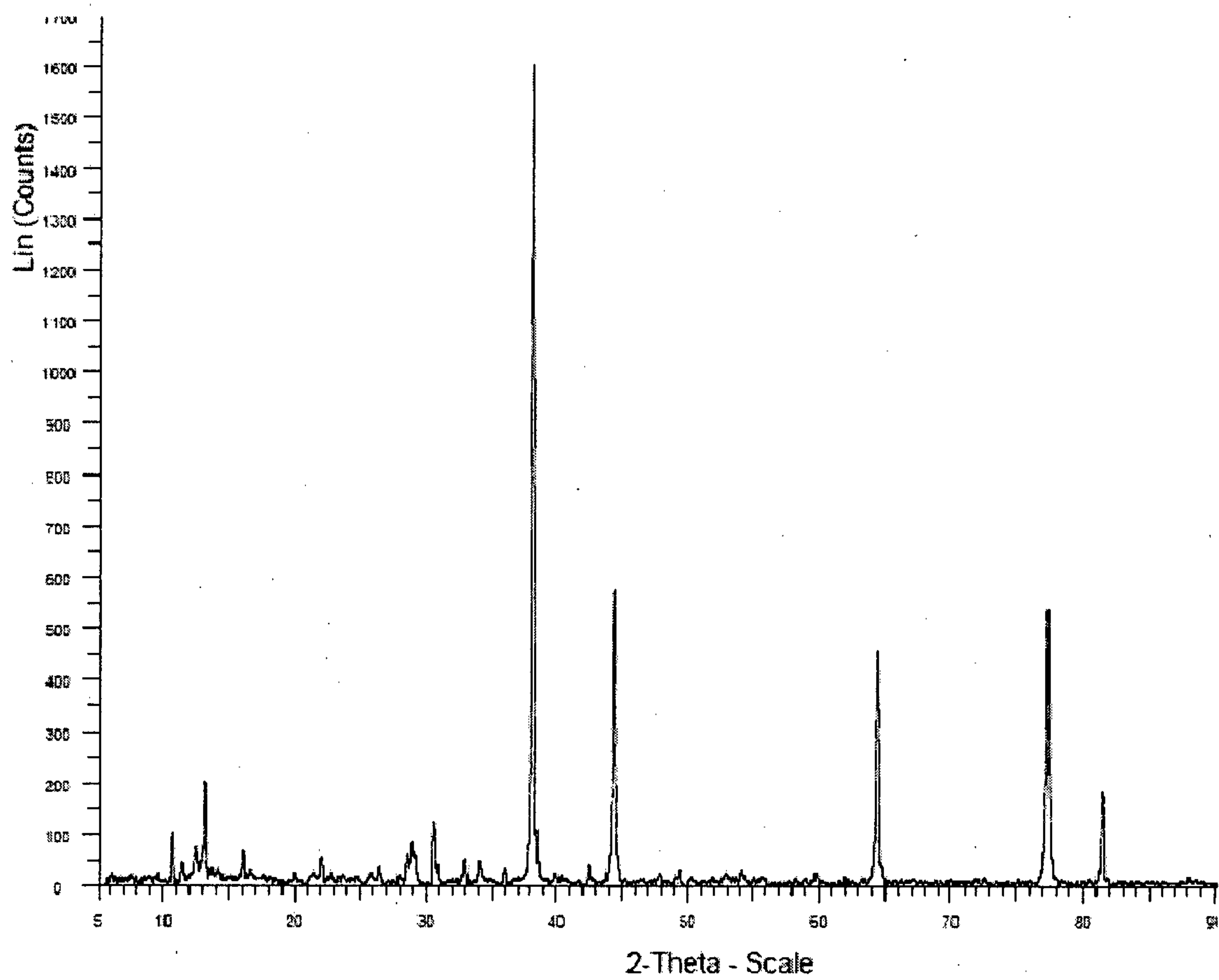
XRD pattern of deposited zinc powder
