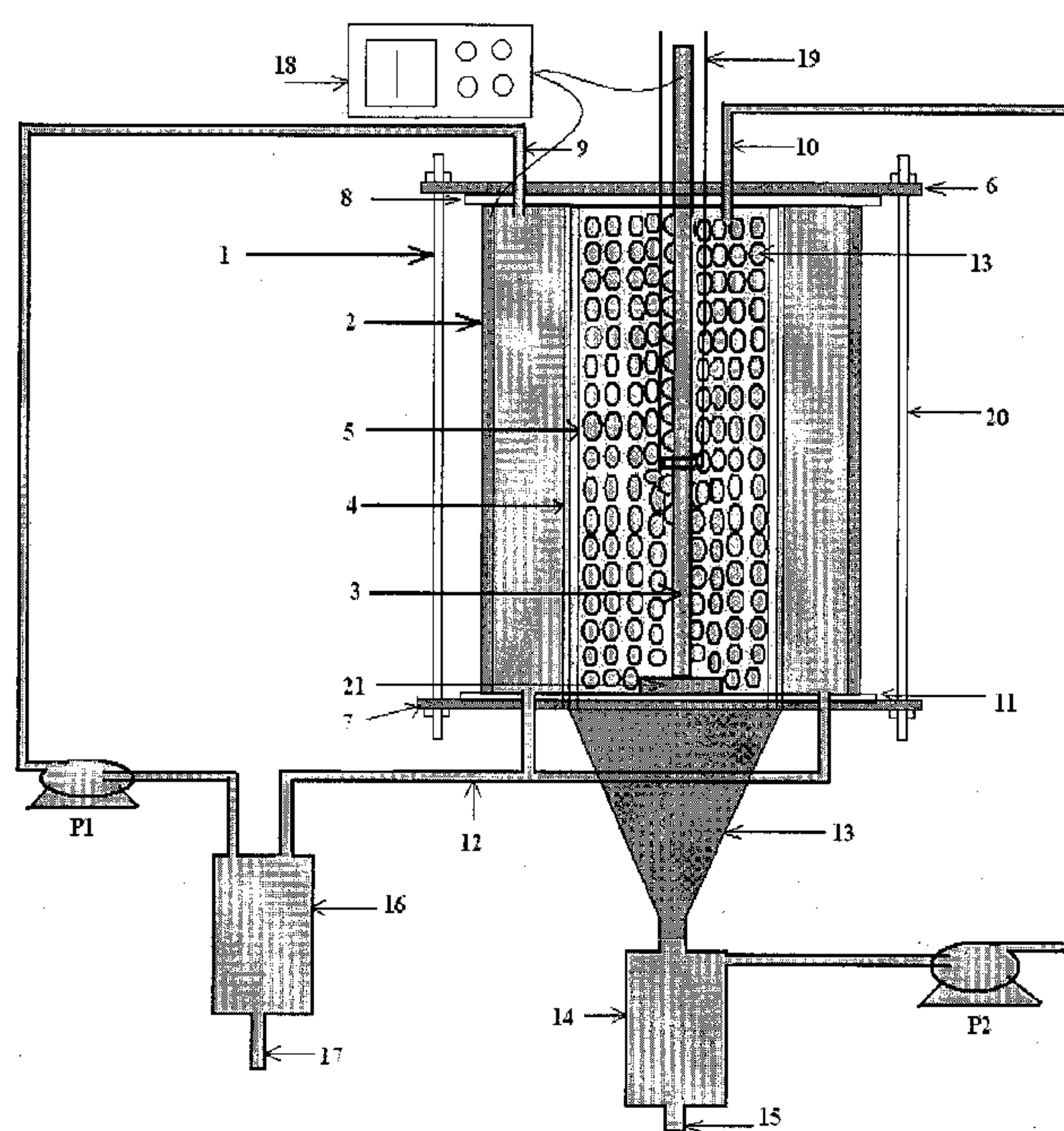
Electrochemical cell for recovery of metals
