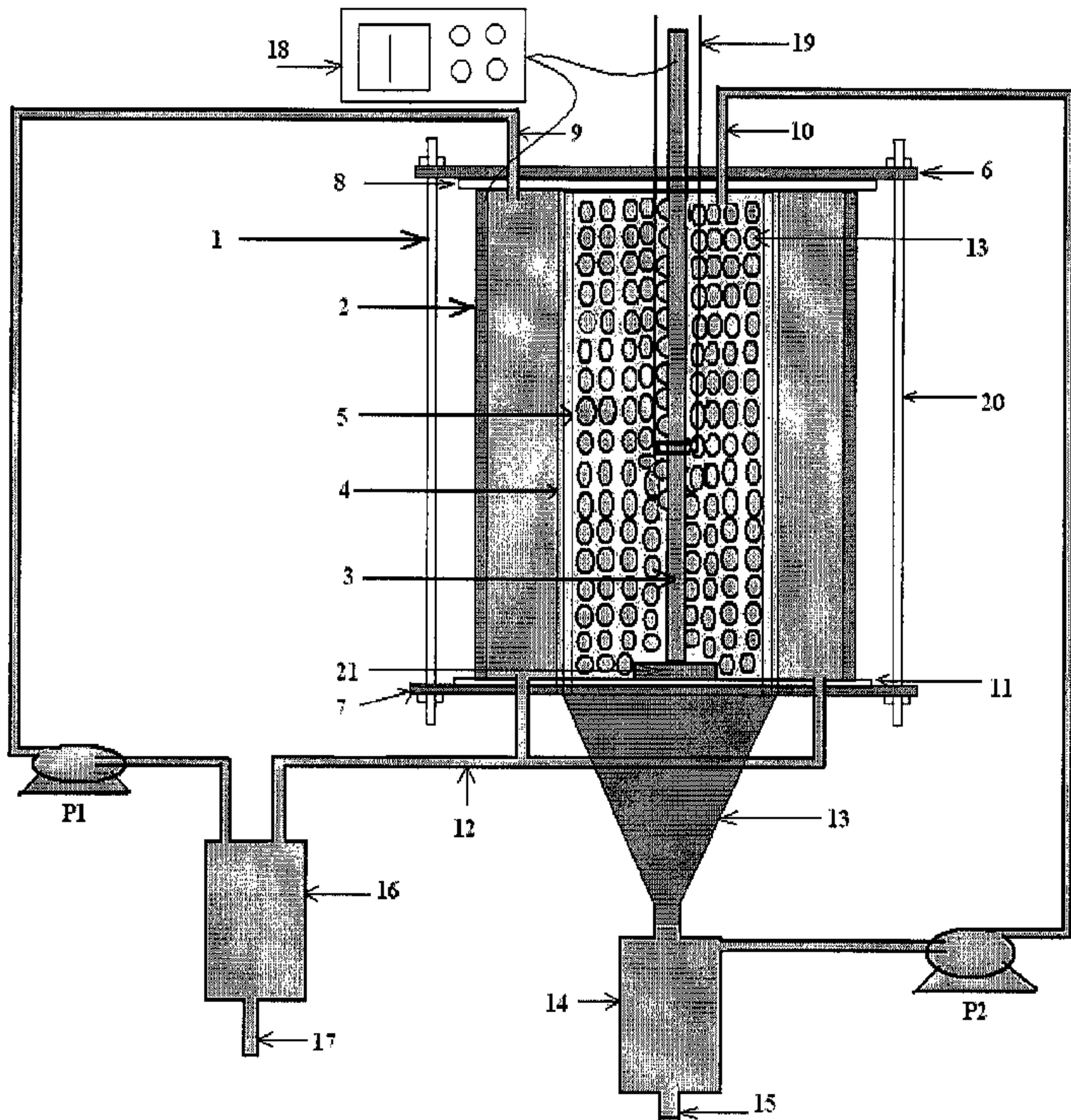
Electrochemical cell for recovery of metals
