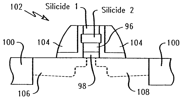
FIG. 5C Post high temp processes:
