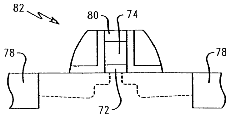
FIG. 4C Post high temp processes:
