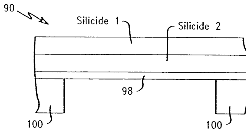
FIG. 5B Post silicide formation:
