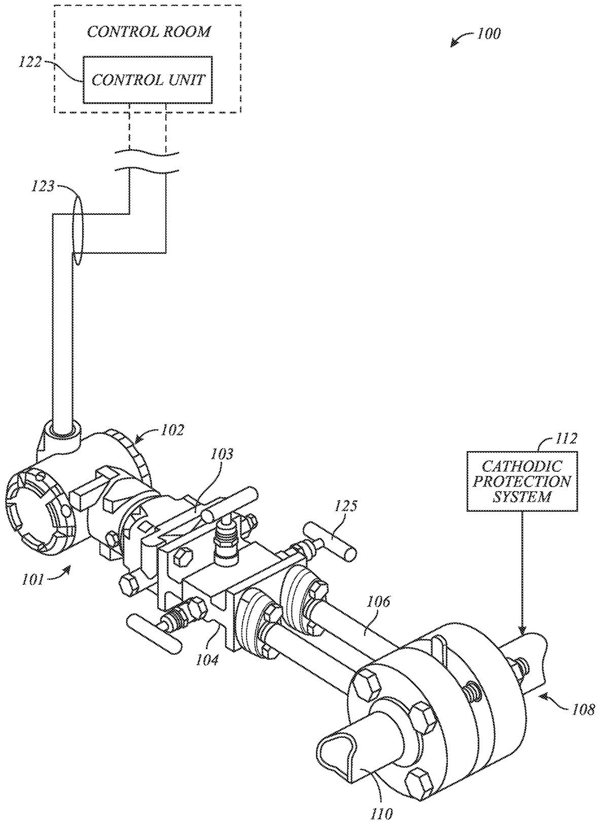
FIG. 1 (Prior Art)
