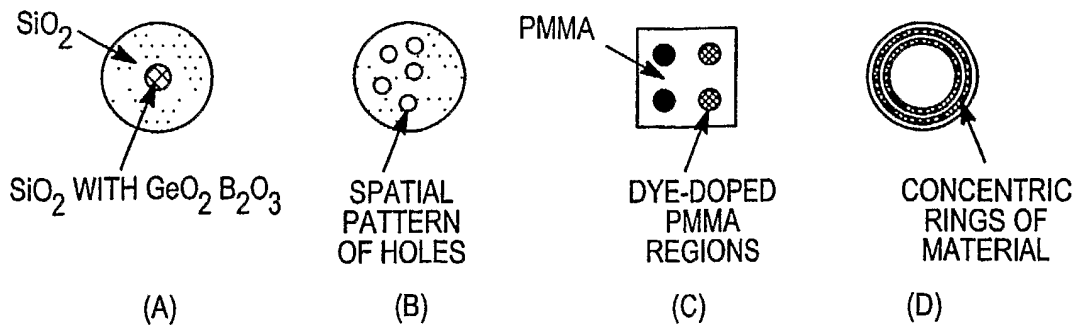
EXAMPLES OF ENCODED PARTICLE CROSS-SECTION BASED ON DIFFERENT CORE GEOMETRIES IN FILAMENT DRAWN AND CUT FROM A PREFORM TO FORM MICROBEADS
