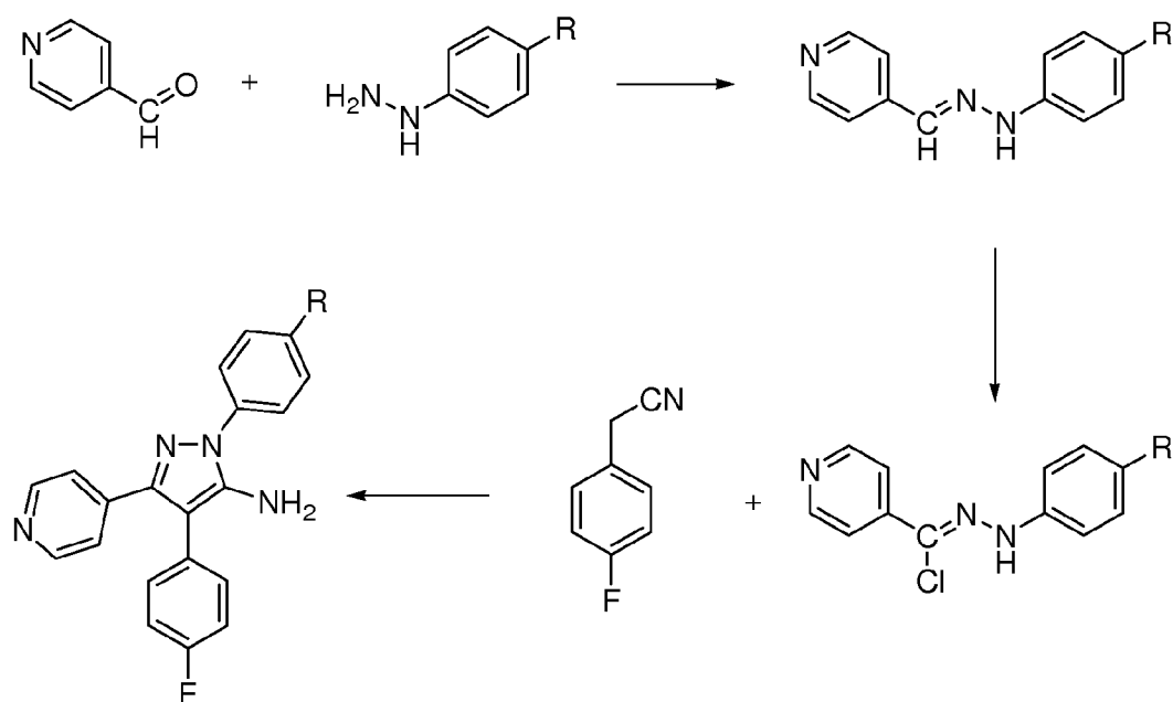
Scheme 1. General methods for pyrazole synthesis
