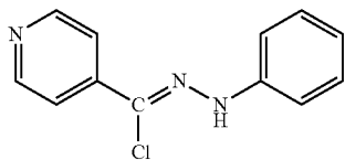
1-(Chloro(pyridin-4-yl)methylene)-2-phenylhydrazine (2)
