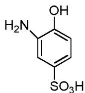
3-amino-4-hydroxybenzenesulfonic acid
