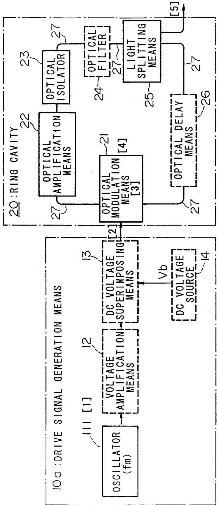
FIG.11 EXAMPLE OF THE COMPOSITION OF A MODE-LOCKED LASER DEVICE OF THE PRIOR ART
