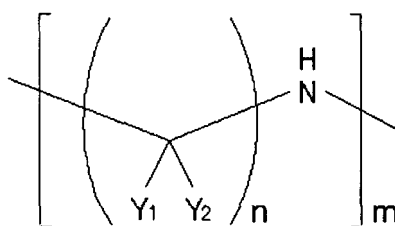
[Chem. Formula 4]
