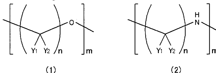
[Chem. Formula 1]
