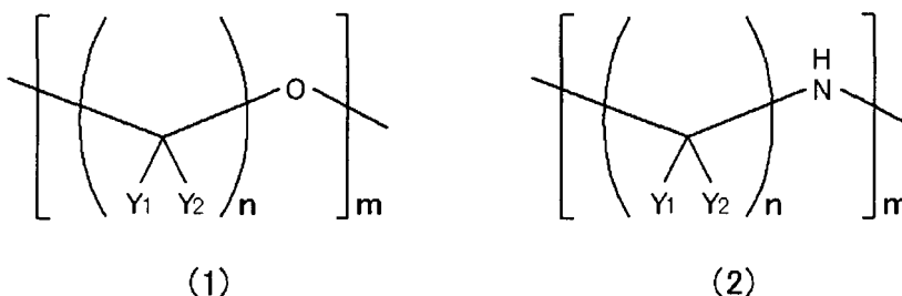
[Chem. Formula 2]
