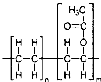
Ethylene-vinyl acetate
