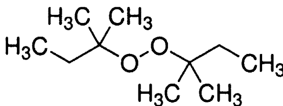
Di-tert-amyl peroxide
