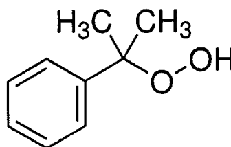
Cumene hydroperoxide
