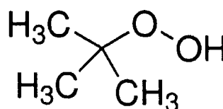
tert-Butyl hydroperoxide
