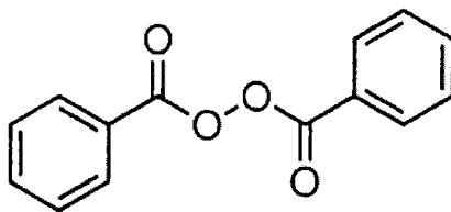
Benzoyl peroxide
