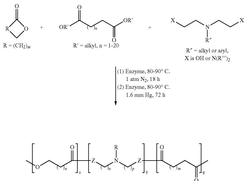
Scheme 1: Preparation of poly(amine-co-ester) terpolymers
