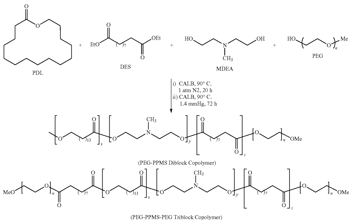
Scheme 2: Enzymatic Synthesis of PEG-PPMS Block Copolymers
