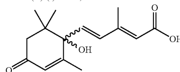
(R,S)-(+)-2-trans-,4-trans-abscisic acid
