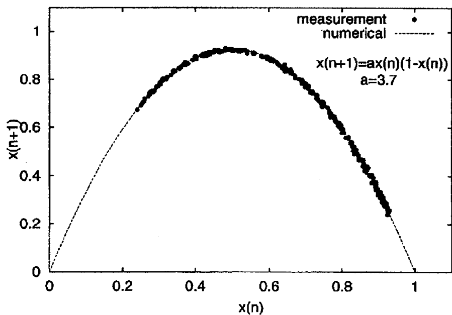
Fig. 24 PRIOR ART
