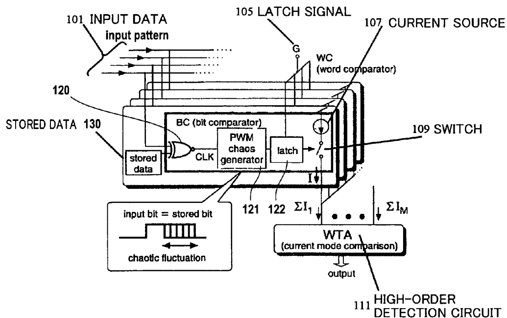
Fig. 23 PRIOR ART
