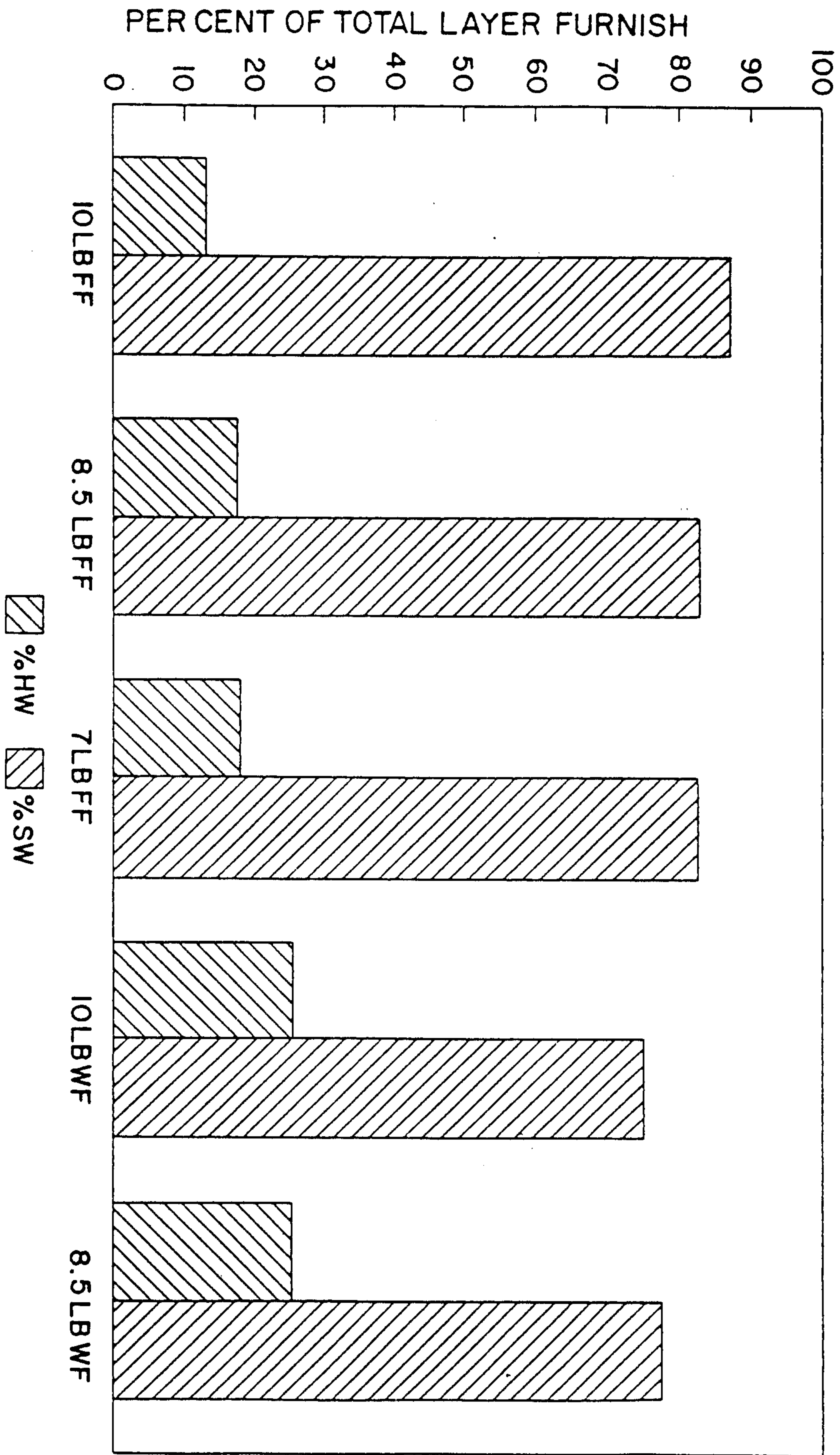
FIG. 6 LAYER PURITY REGION 8 (AIR SIDE)
