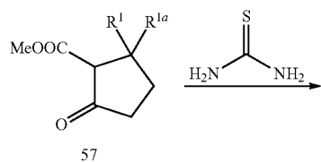
Scheme 7
