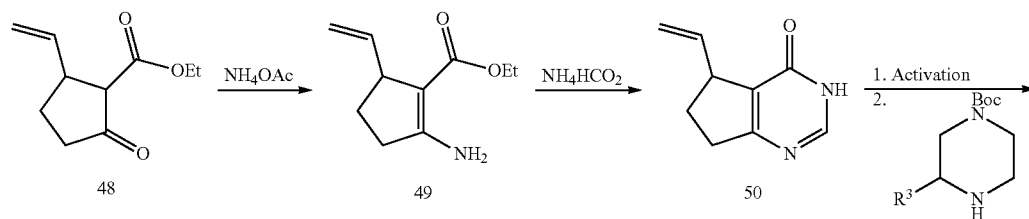
Scheme 6
