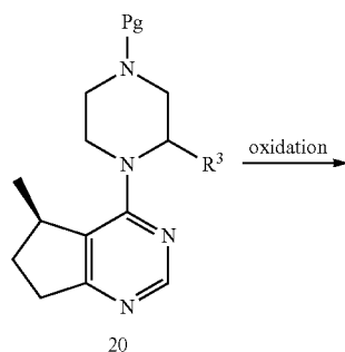
Scheme 3
