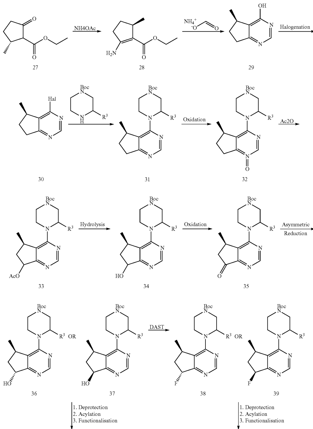
Scheme 4
