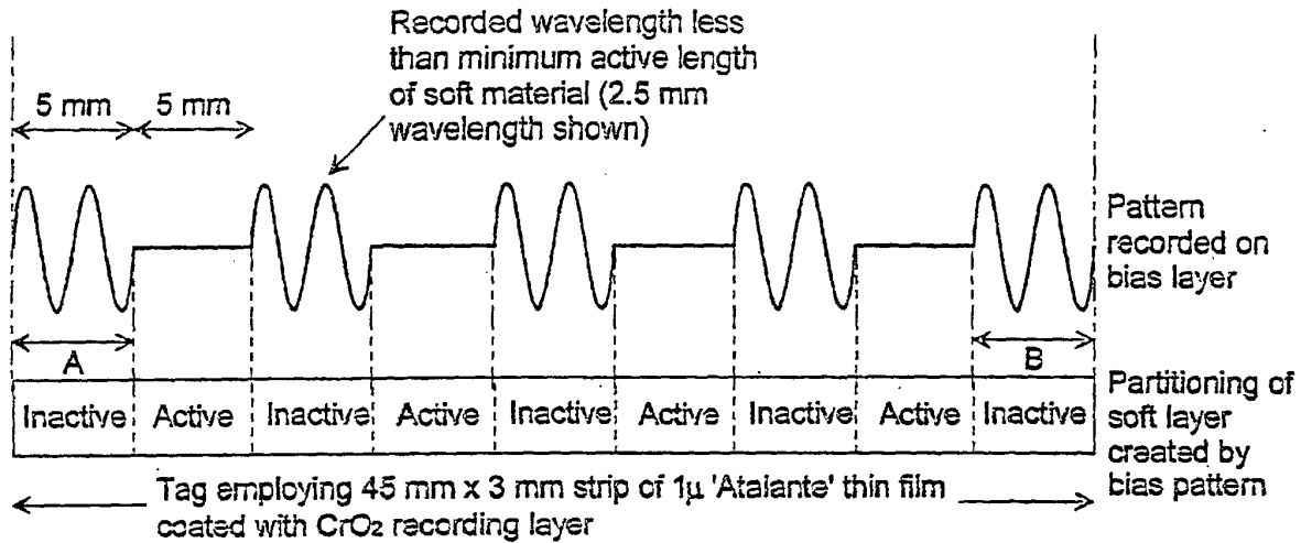
Fig 1: Example of recorded pattern to magnetically partition 45mm strip tag into 4 active segments
