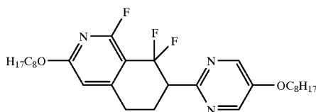
7-[5-(Octyloxy)pyrimidin-2-yl]-1,8,8-trifluoro-3-octyloxy-5,6,7,8-tetrahydroisoquinoline
