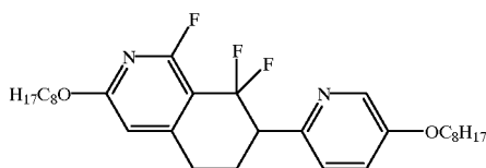
7-[5-(Octyloxy)pyridin-2-yl]-1,8,8-trifluoro-3-octyloxy-5,6,7,8-tetrahydroiso-quinoline
