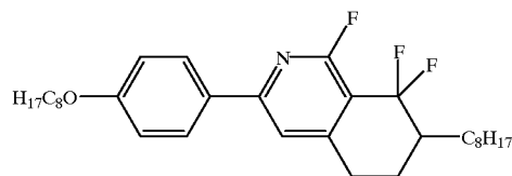
1,8,8-Trifluoro-3-[4-(octyloxy)phenyl]-7-octyl-5,6,7,8-tetrahydroisoquinoline
