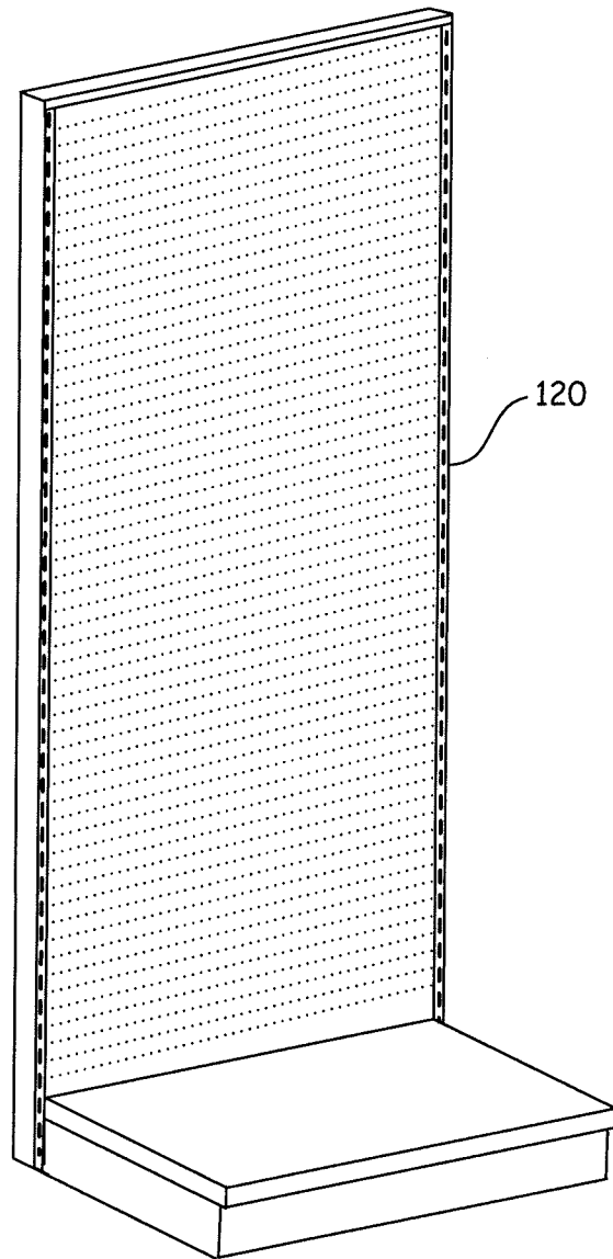
FIG. 14 (PRIOR ART)
