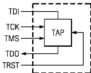
FIG. 4A (PRIOR ART)
