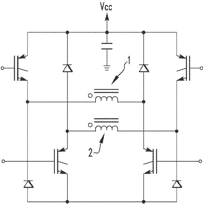
FIG. 2 (PRIOR ART)
