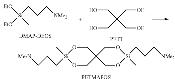
Figure 3. Synthesis of PETMAPOS
