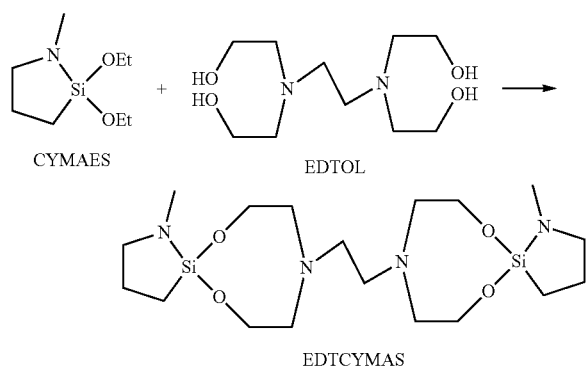
Figure 4. Synthesis of EDTCYMAS
