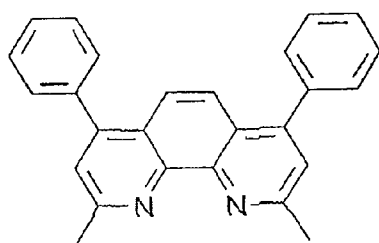
BCP= Bathocuproin (2,9-Dimethyl-4,7-Diphenyl- 1,10-phenanthroline) C 26 H 20 N 2
