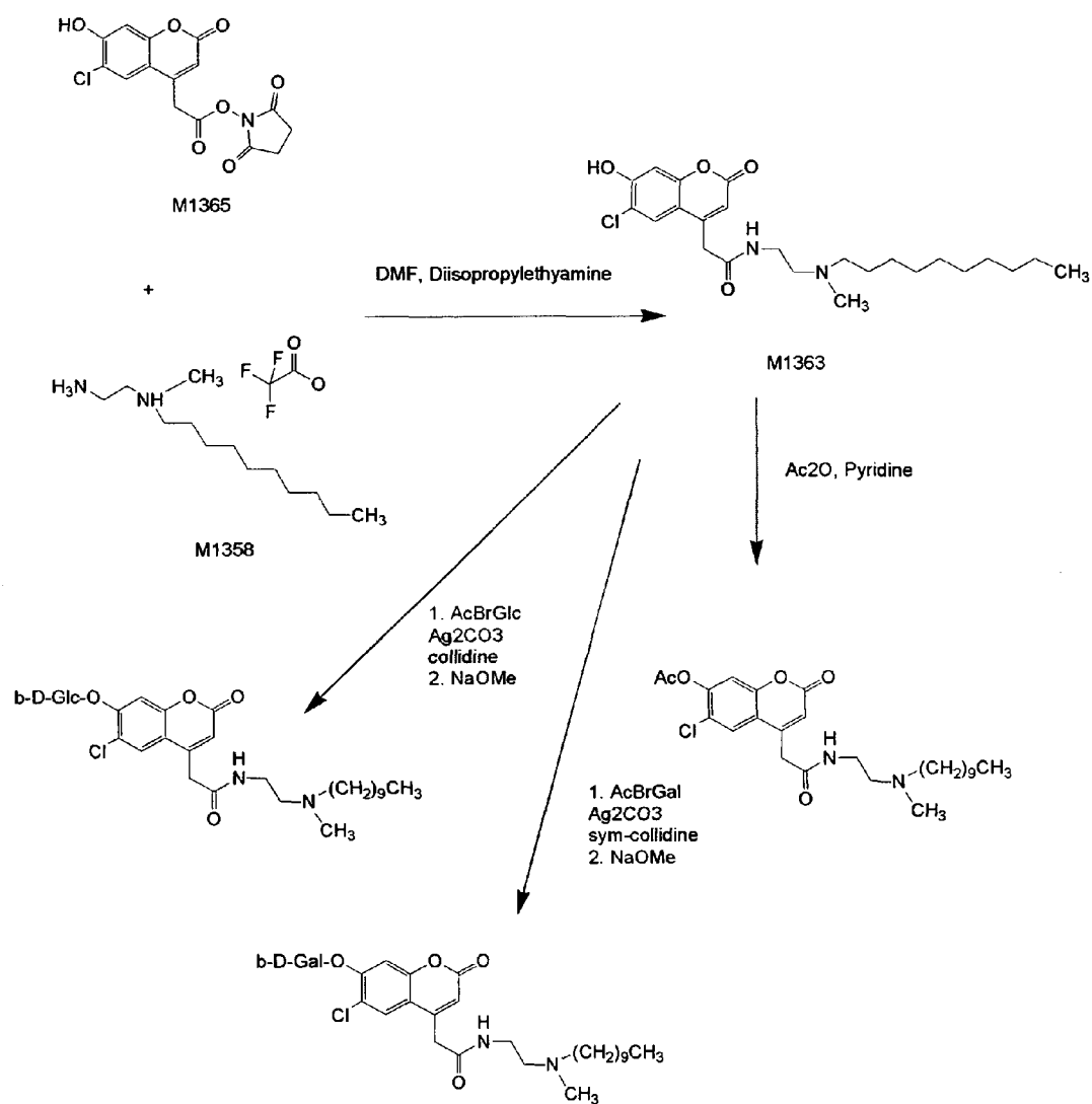
Figure 10: Lipophilic Targeting Group Esterase and Glycosidase Substrate Syntheses.
