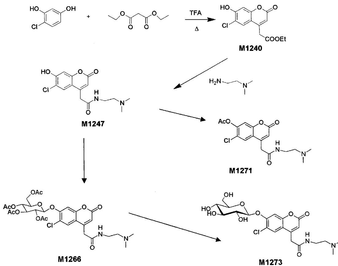
Figure 3. Coumarin based probes. (blue fluorescence)
