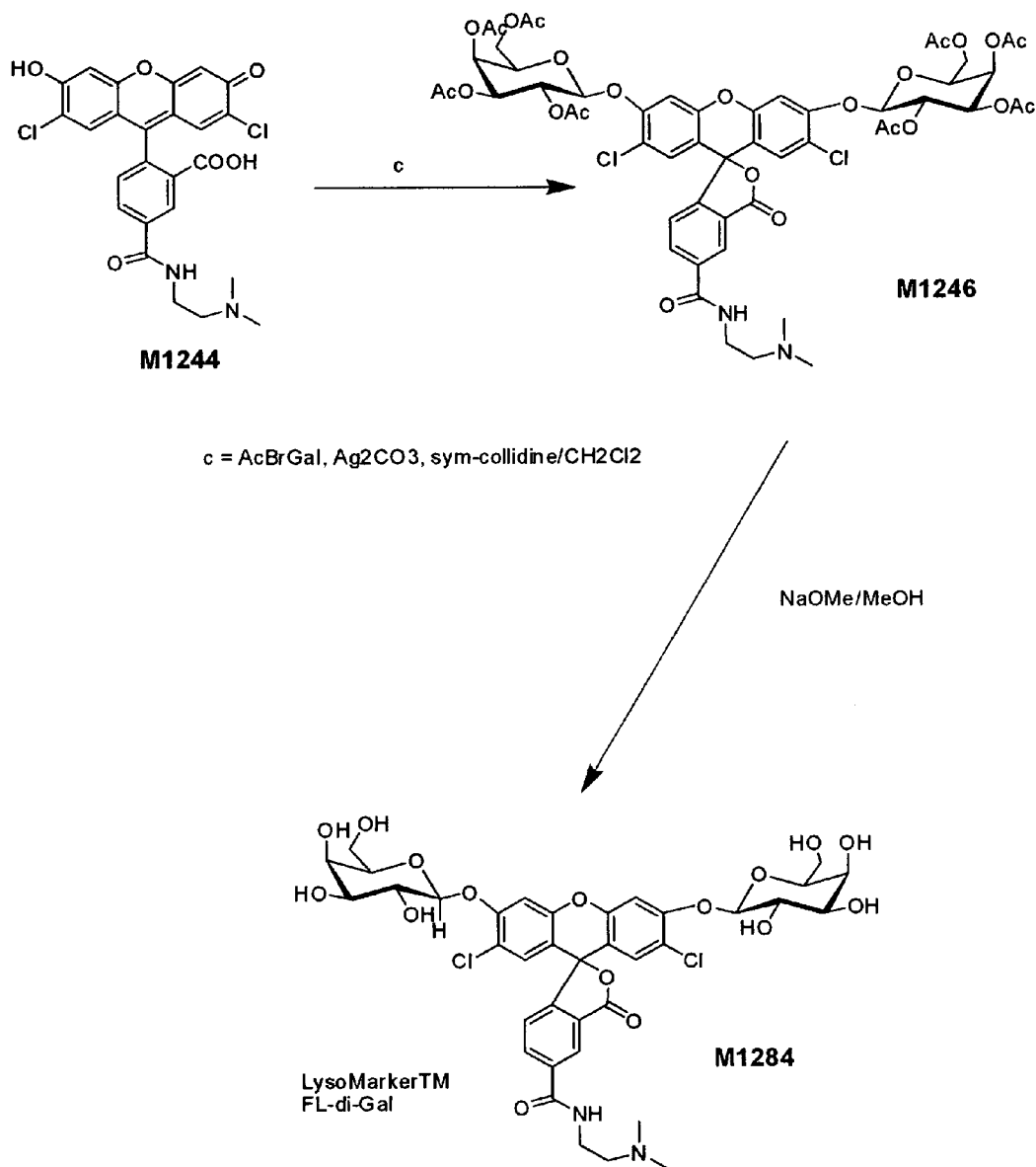
Figure 2. Krabbe LysoMarker™ Substrates.
