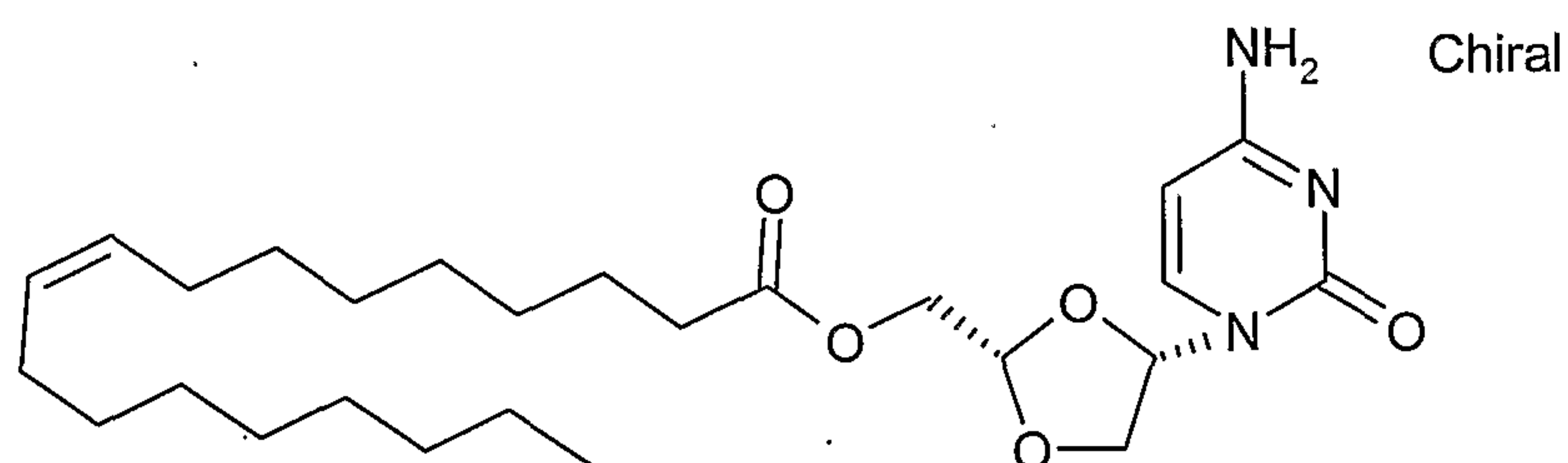
COMPOUND #21
