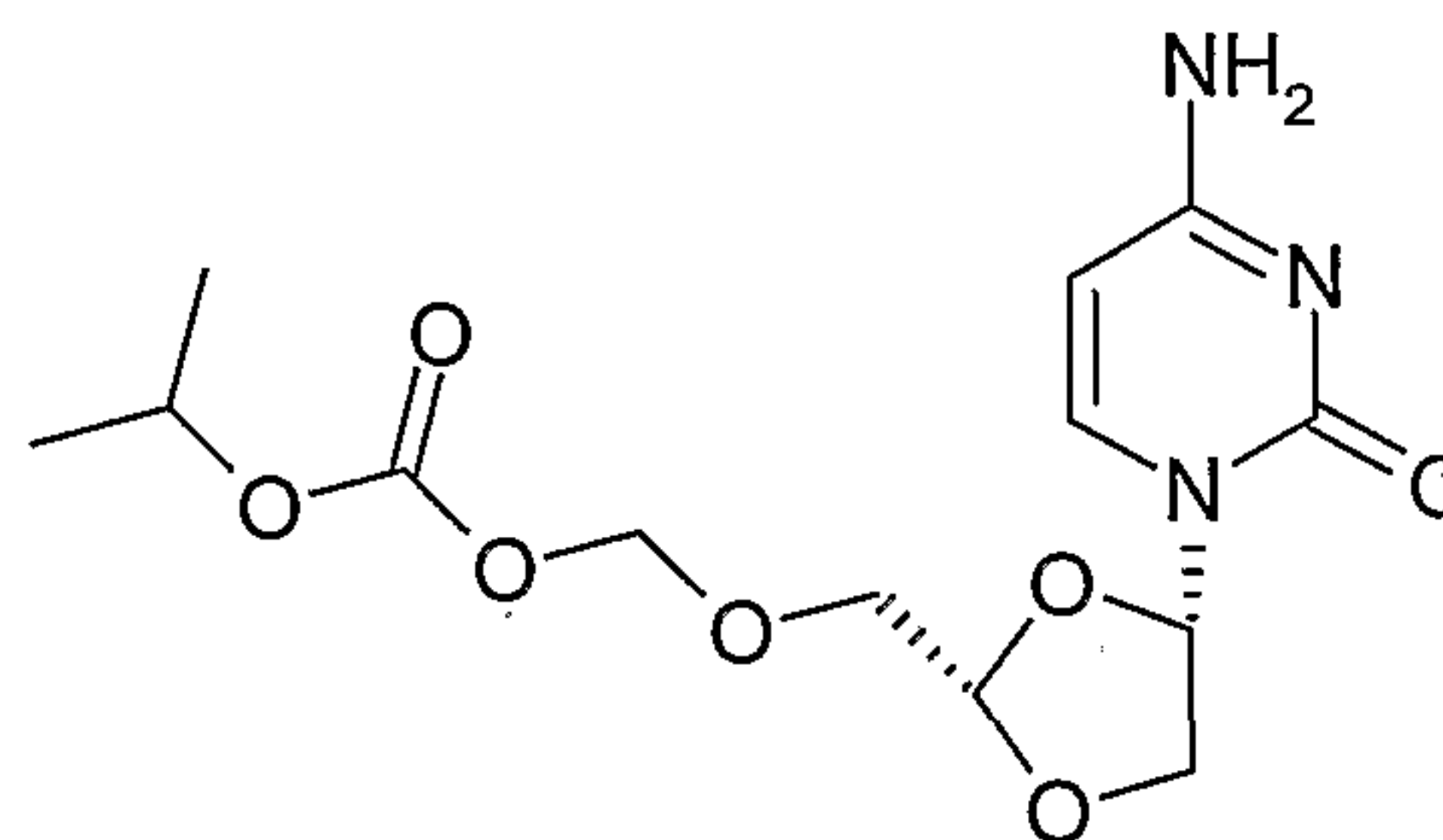
Carbonic acid 4-(4-amino-2- oxo-2H-pyrimidin-1-yl)-[1,3] dioxolan-2-ylmethoxymethyl ester isopropyl ester
