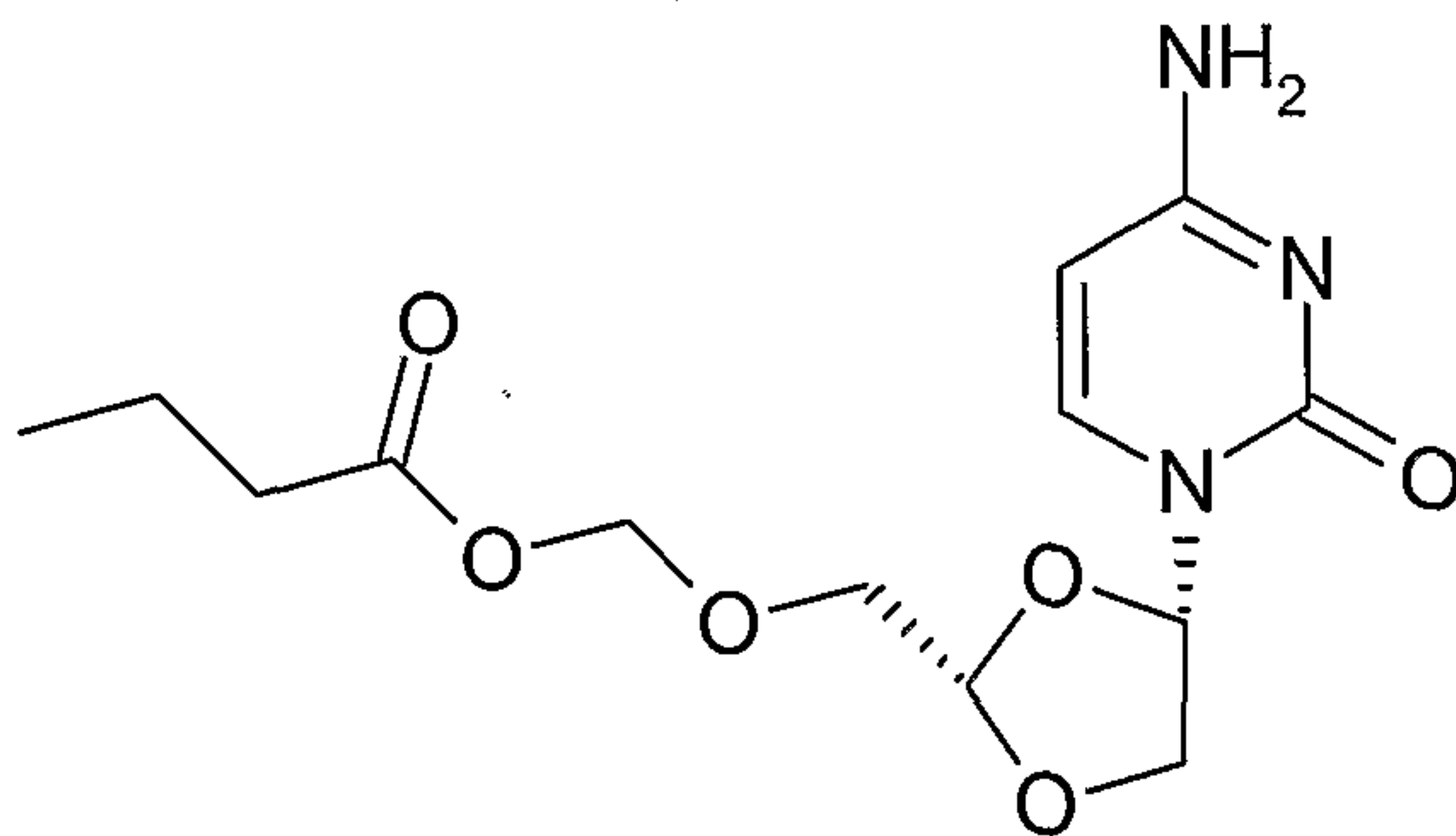
Butyric acid 4-(4-amino-2-oxo-2H-pyrimidin-1-yl)-[1,3]dioxolan-2-ylmethoxymethyl ester
