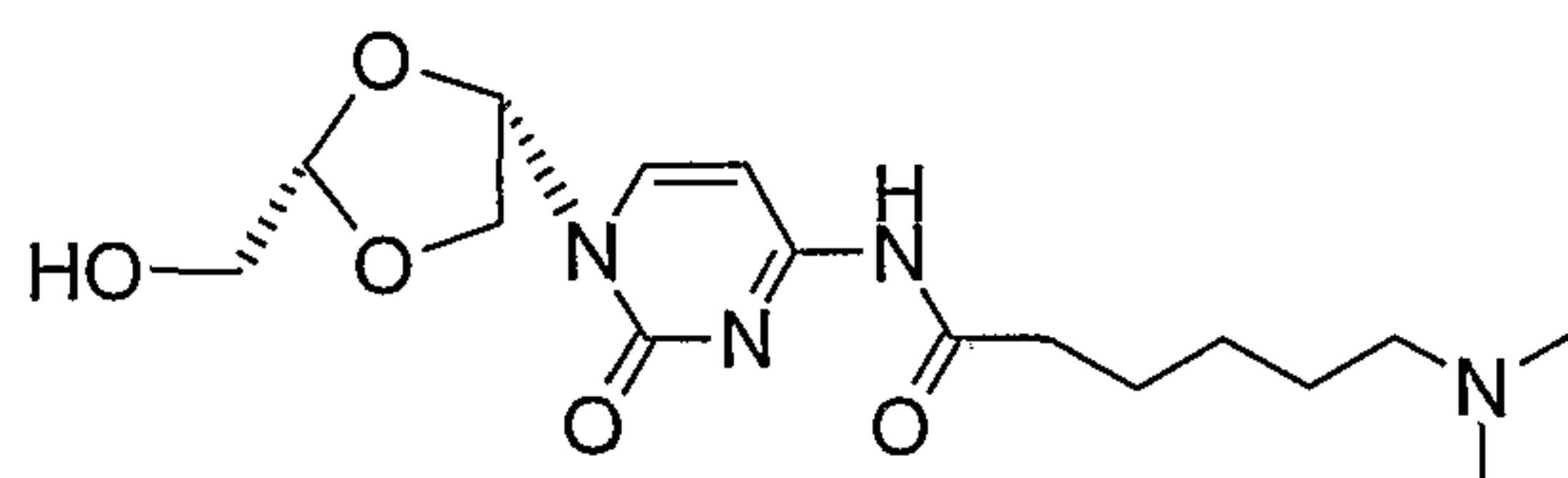
7-Dimethylamino-heptanoic acid [1-(2-hydroxymethyl-[1,3]dioxolan-4-yl)-2-oxo-1,2-dihydro-pyrimidin-4-yl]-amide
