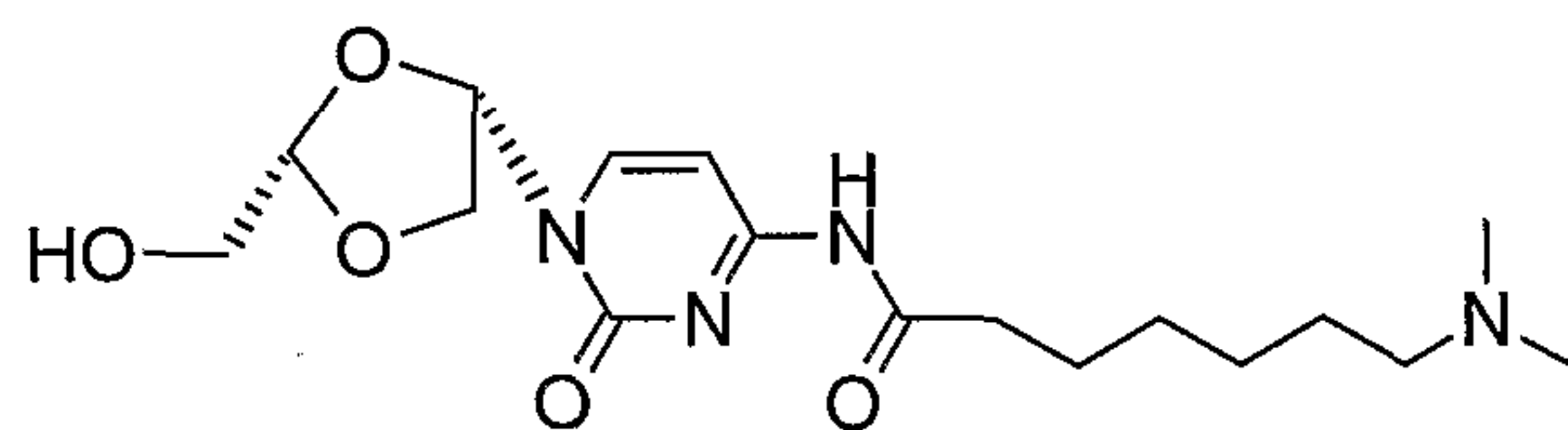
7-Dimethylamino-heptanoic acid [1-(2-hydroxymethyl-[1,3]dioxolan-4-yl)-2-oxo-1,2-dihydro-pyrimidin-4-yl]-amide
