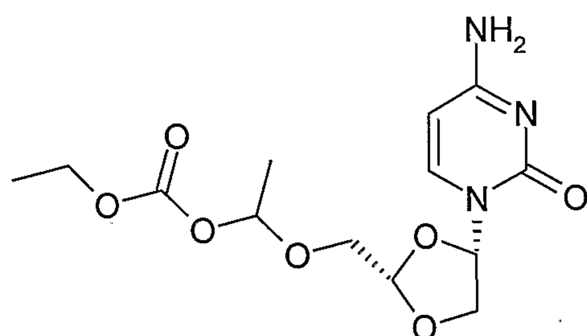
Carbonic acid 1-[4-(4-amino- 2-oxo-2H-pyrimidin-1-yl)- [1,3]dioxolan-2-ylmethoxy]- ethyl ester ethyl ester
