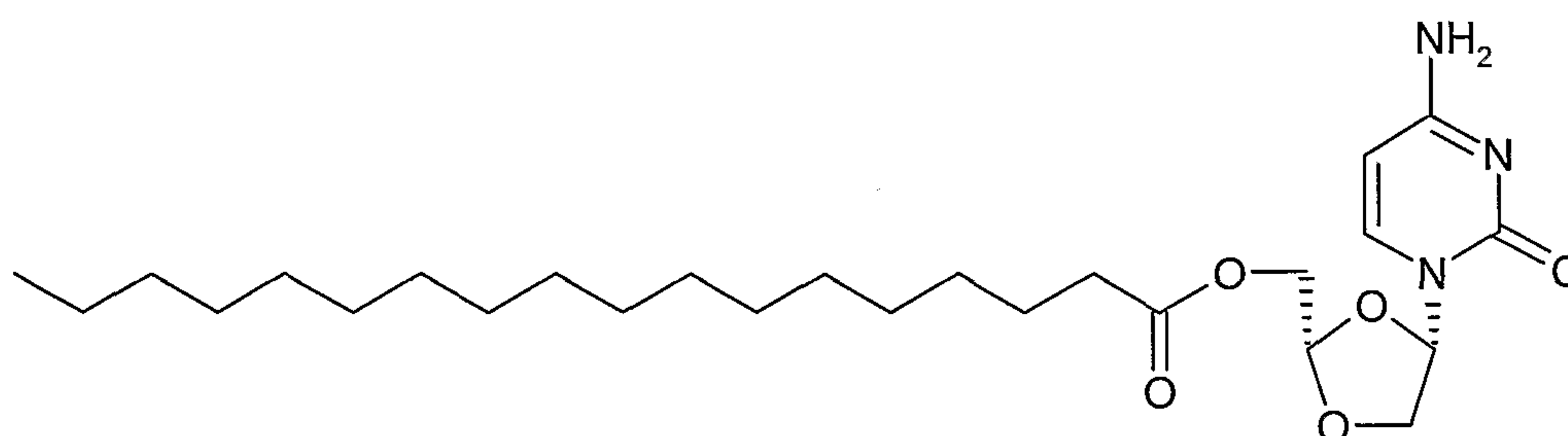
COMPOUND #20
