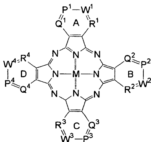
Formula (V)
