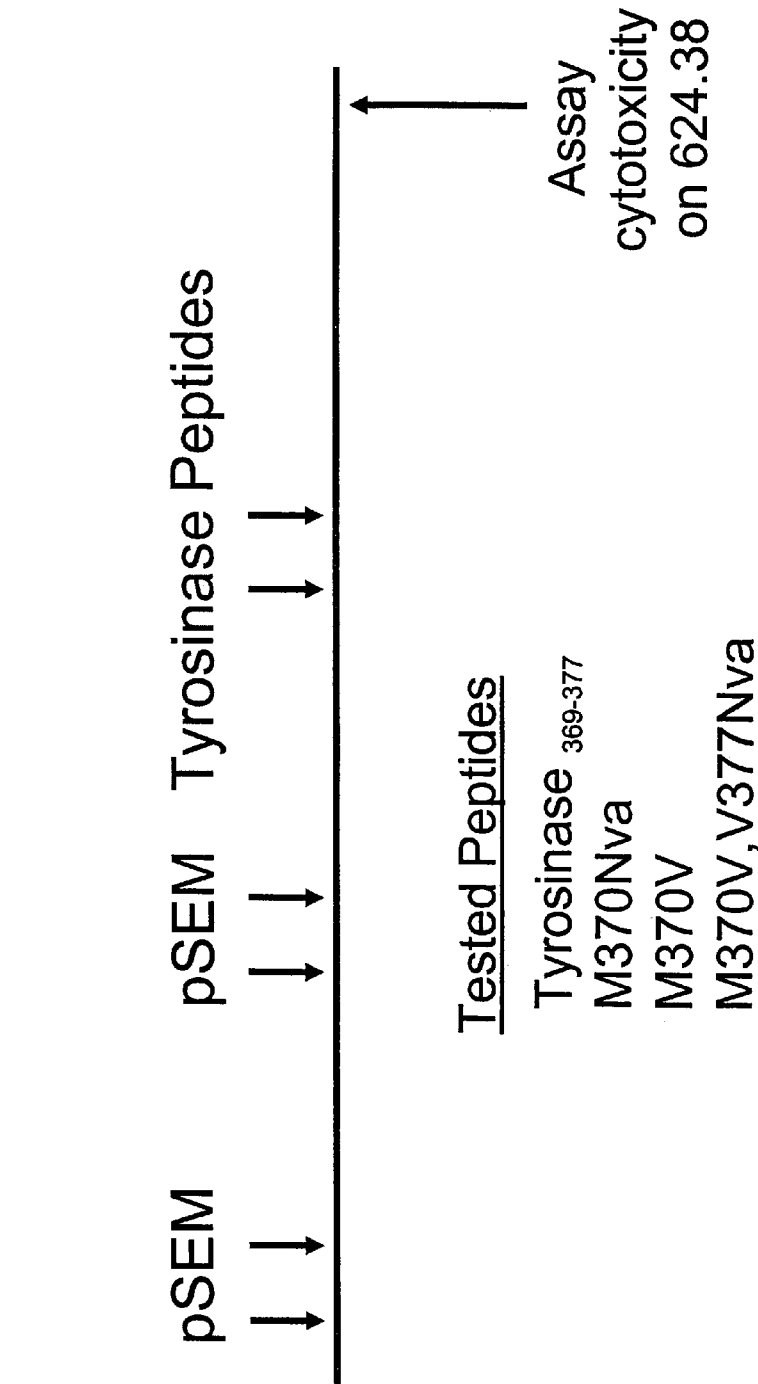
Figure 40: Schematic of Analog Immunogenicity Evaluation Protocol
