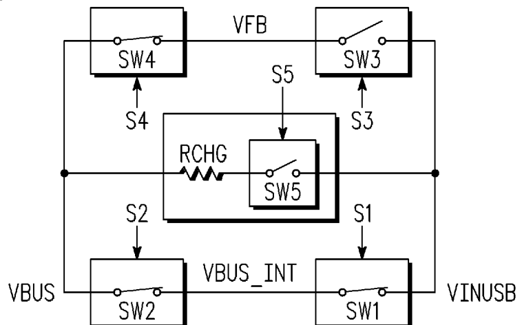
FIG. 6 (USB HOST MODE)
