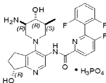
Compound 1 phosphoric acid salt
