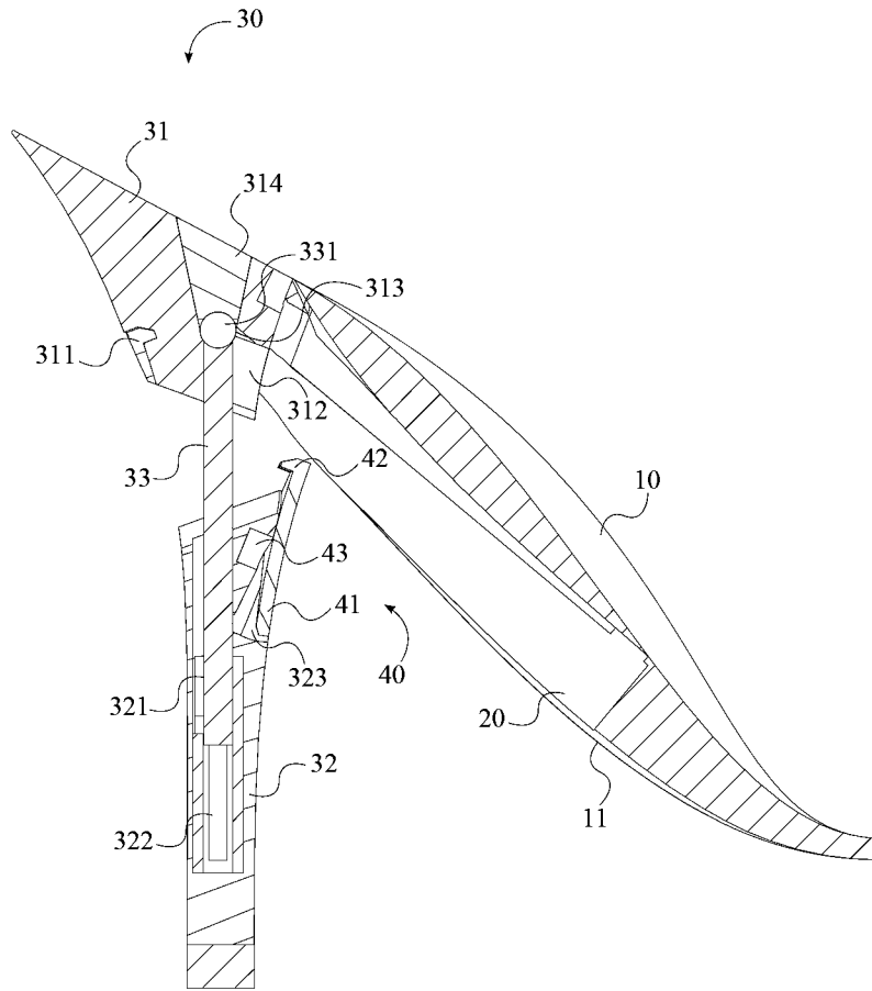
SECTION C-C
