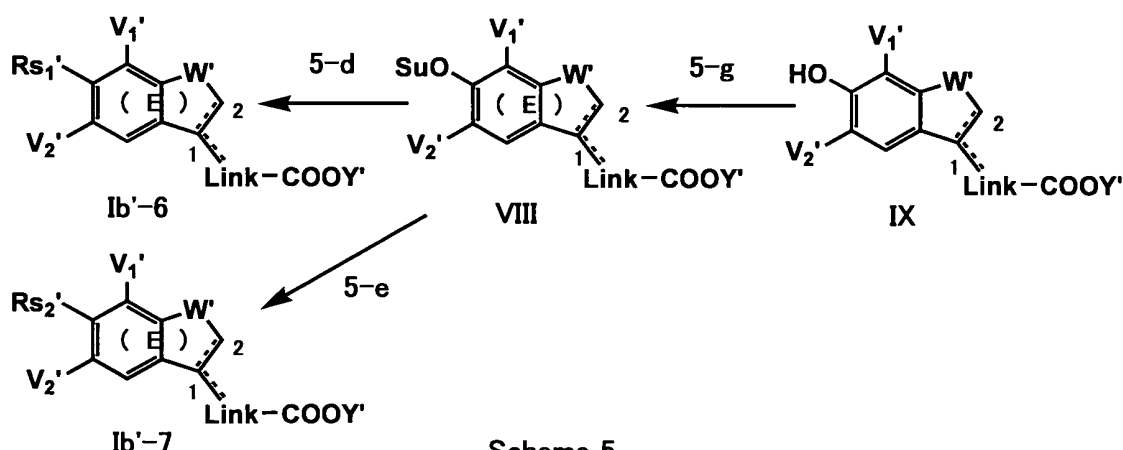
Scheme 5
