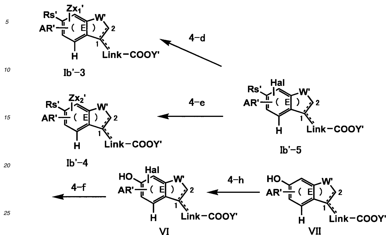
Scheme 4
