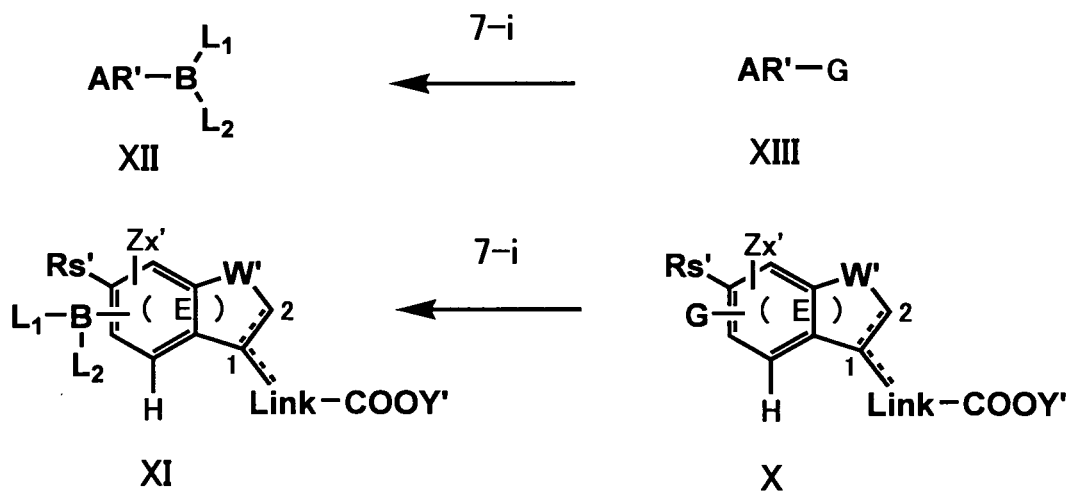
Scheme 7
