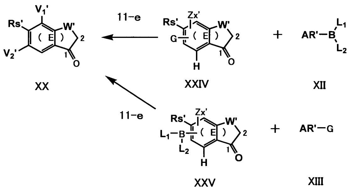
Scheme 11
