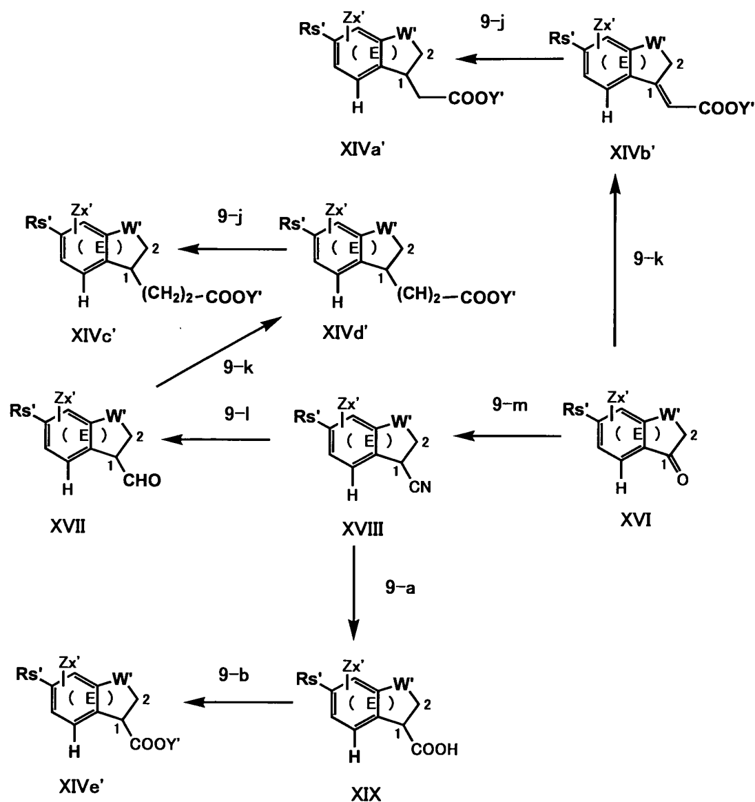
Scheme 9
