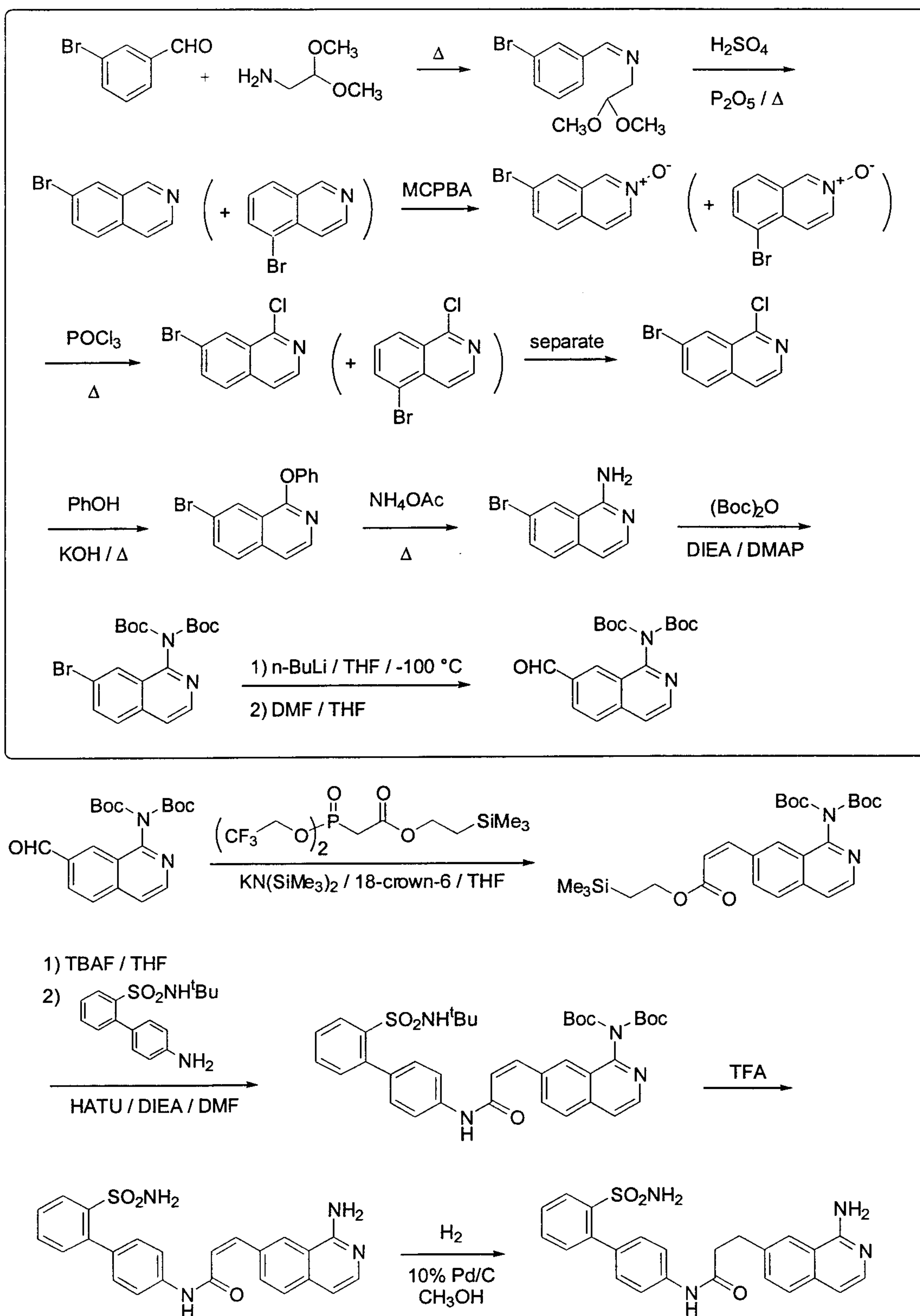
Scheme 10
