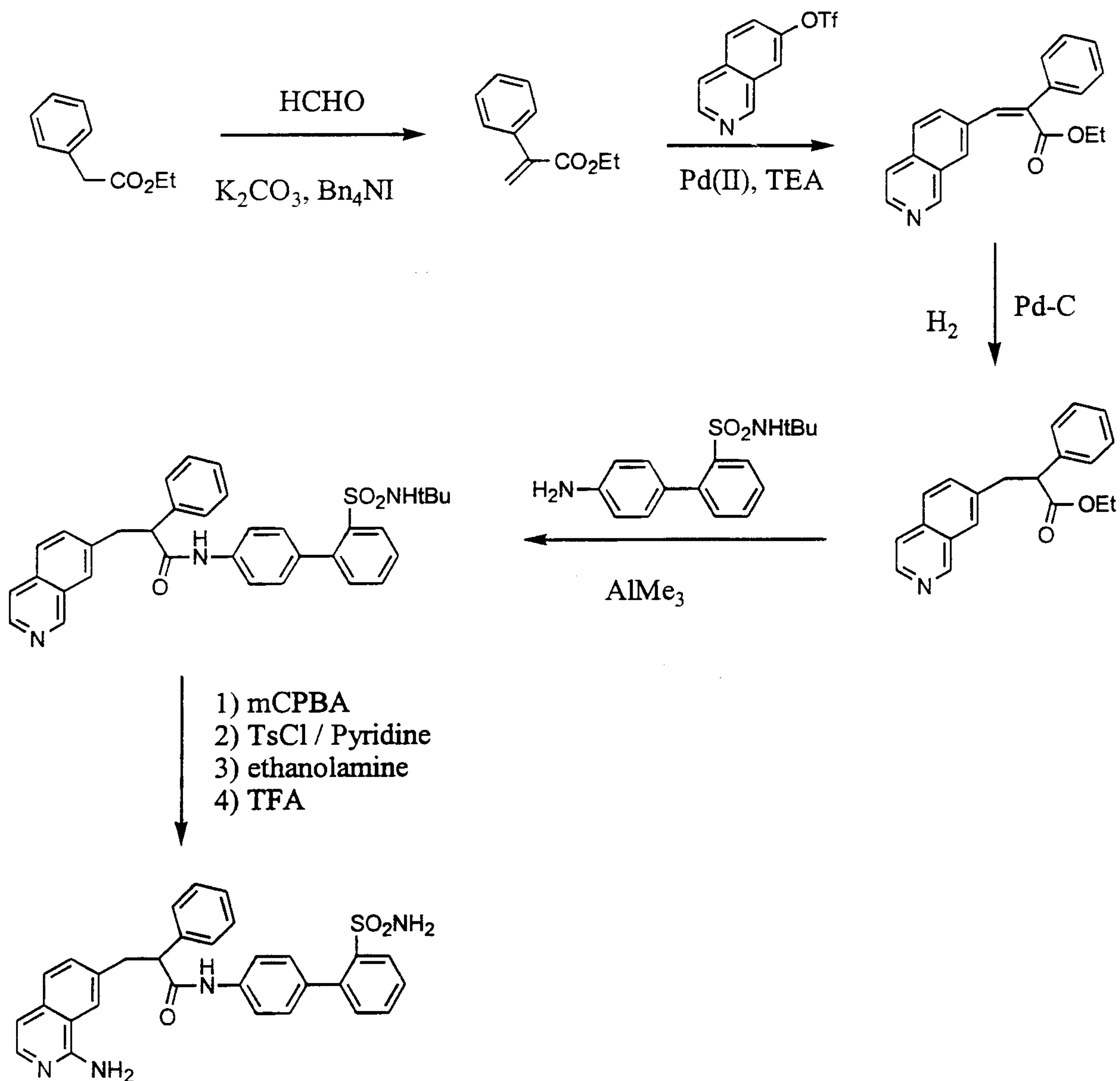
Scheme 12
