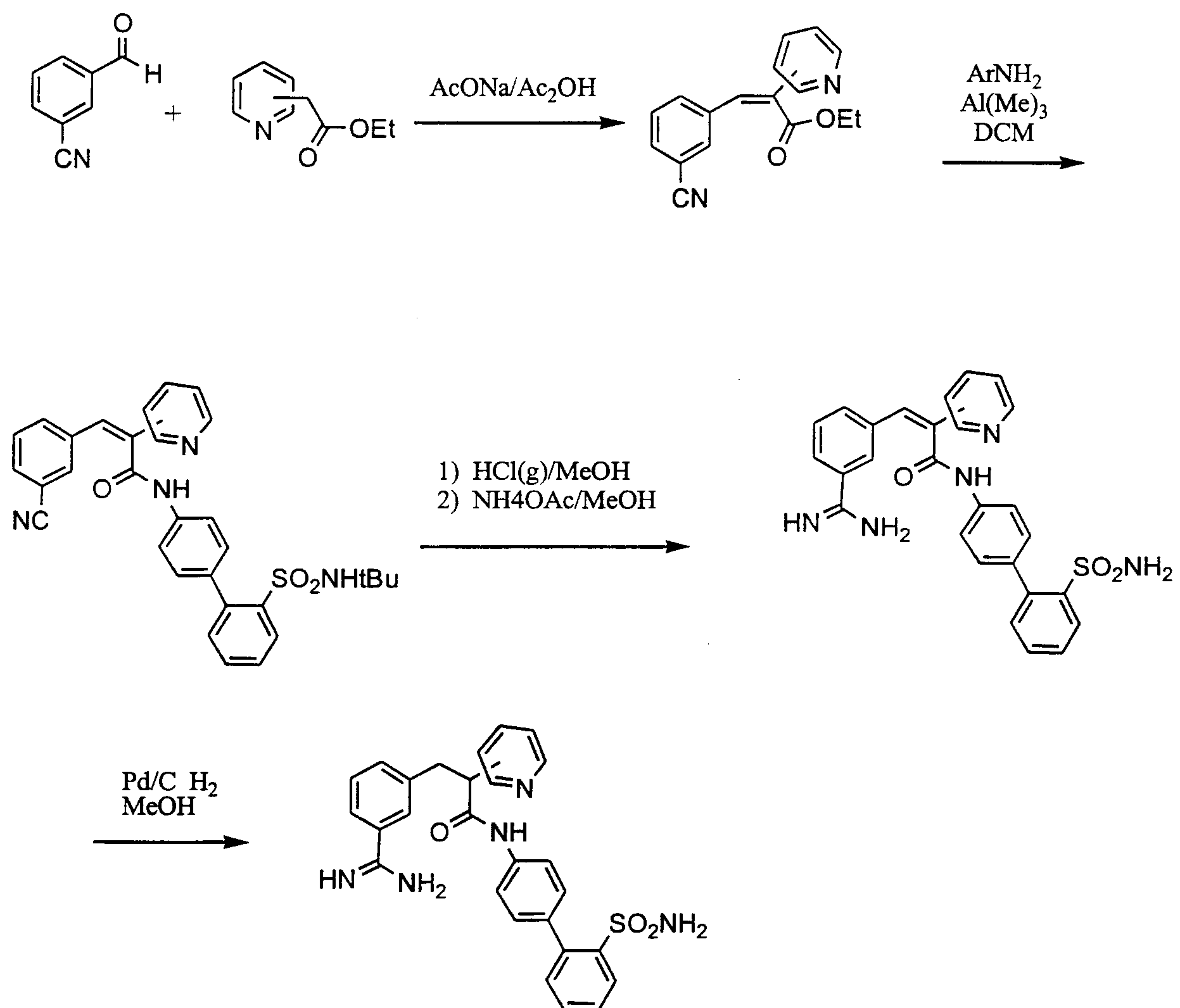
Scheme 8
