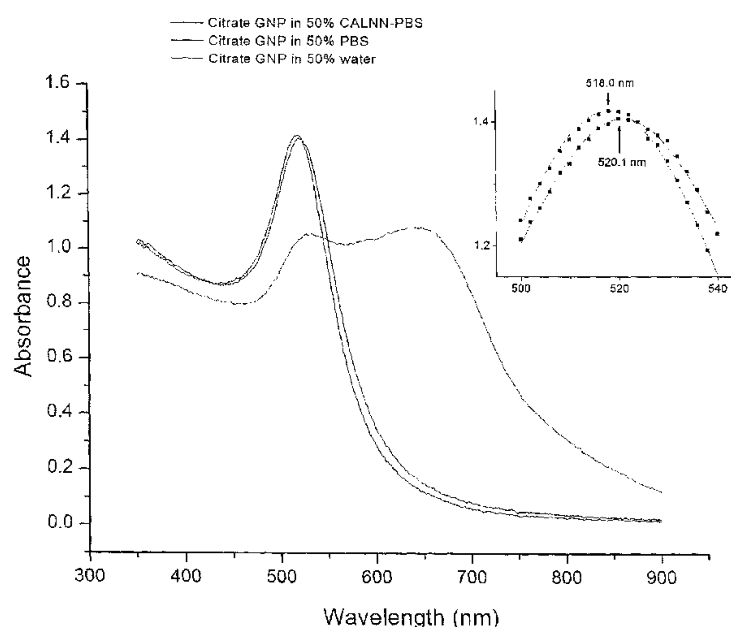
Rapid stabilisation of citrate gold nanoparticles
