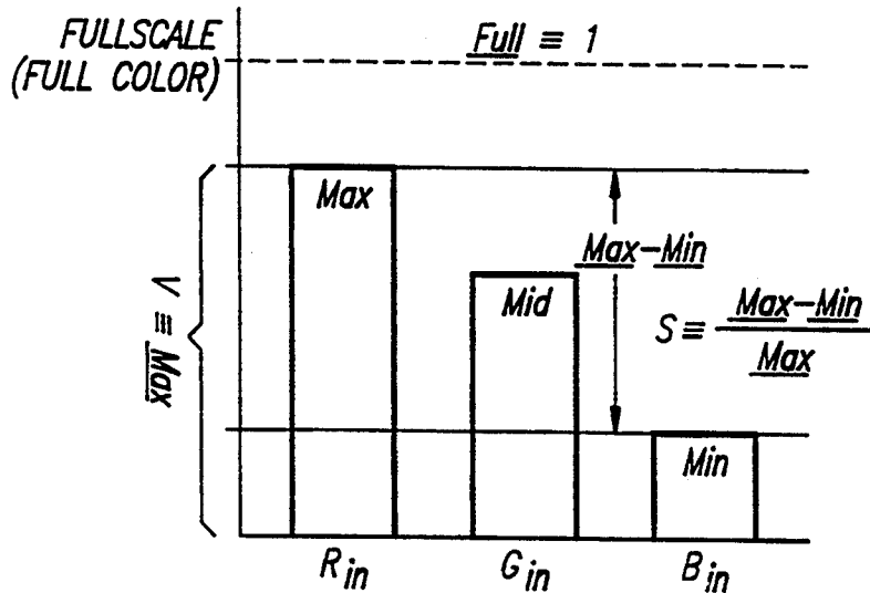
FIG. 6 PRIOR ART
