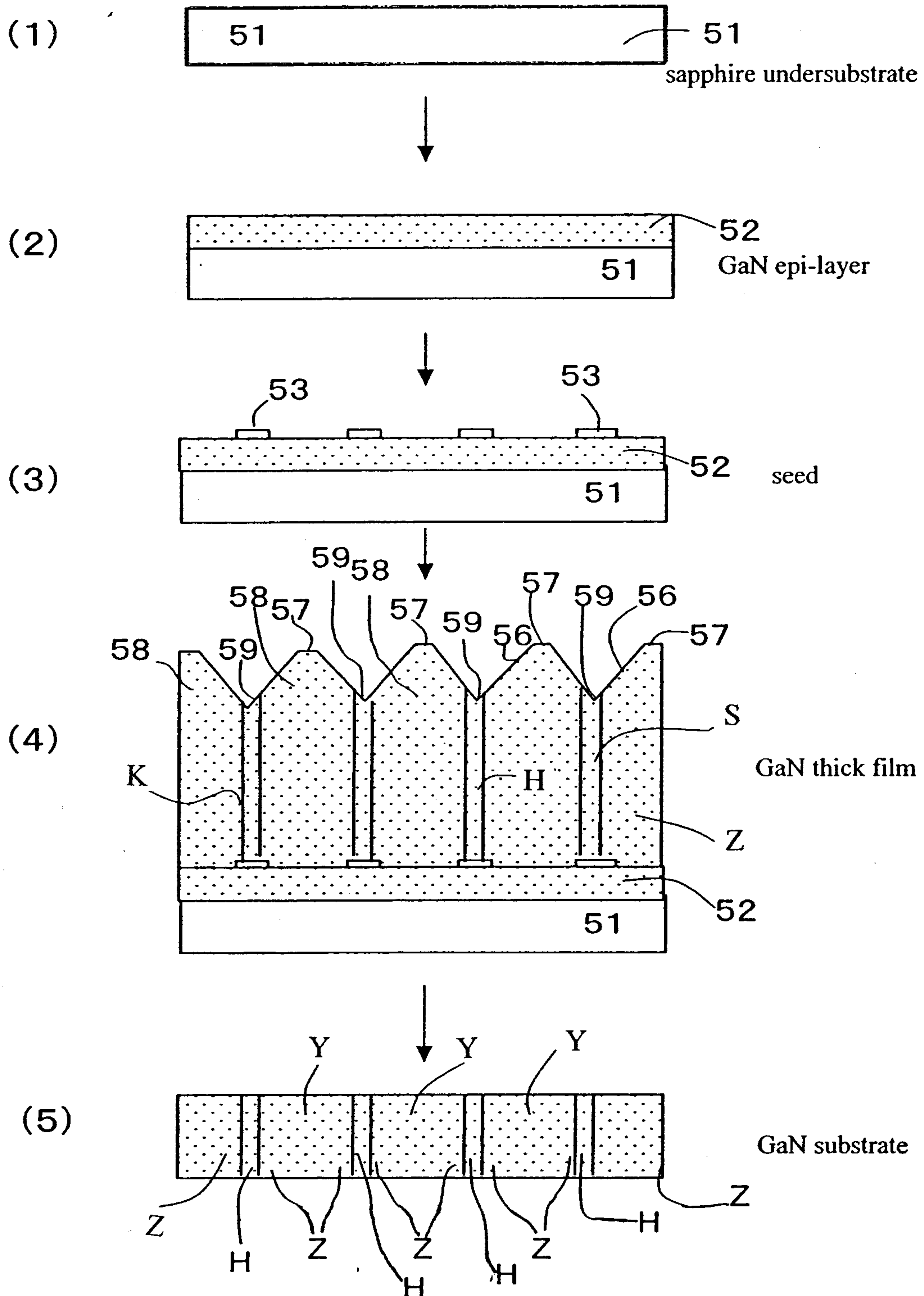
Embodiment 1 Fig.11 Processes of producing a GaN substrate
