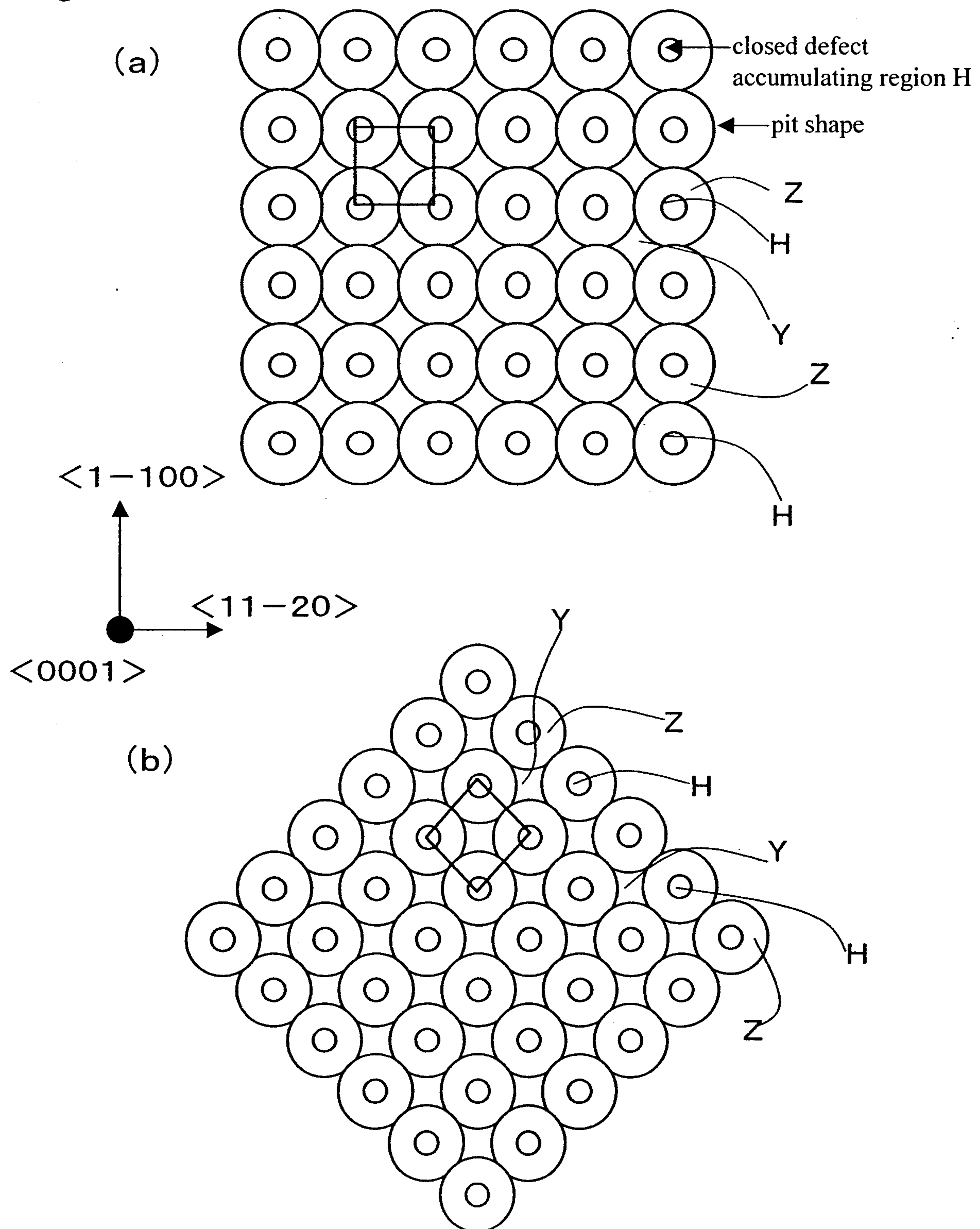
Fig.9 four-fold rotational arrangement on undersubstrate
