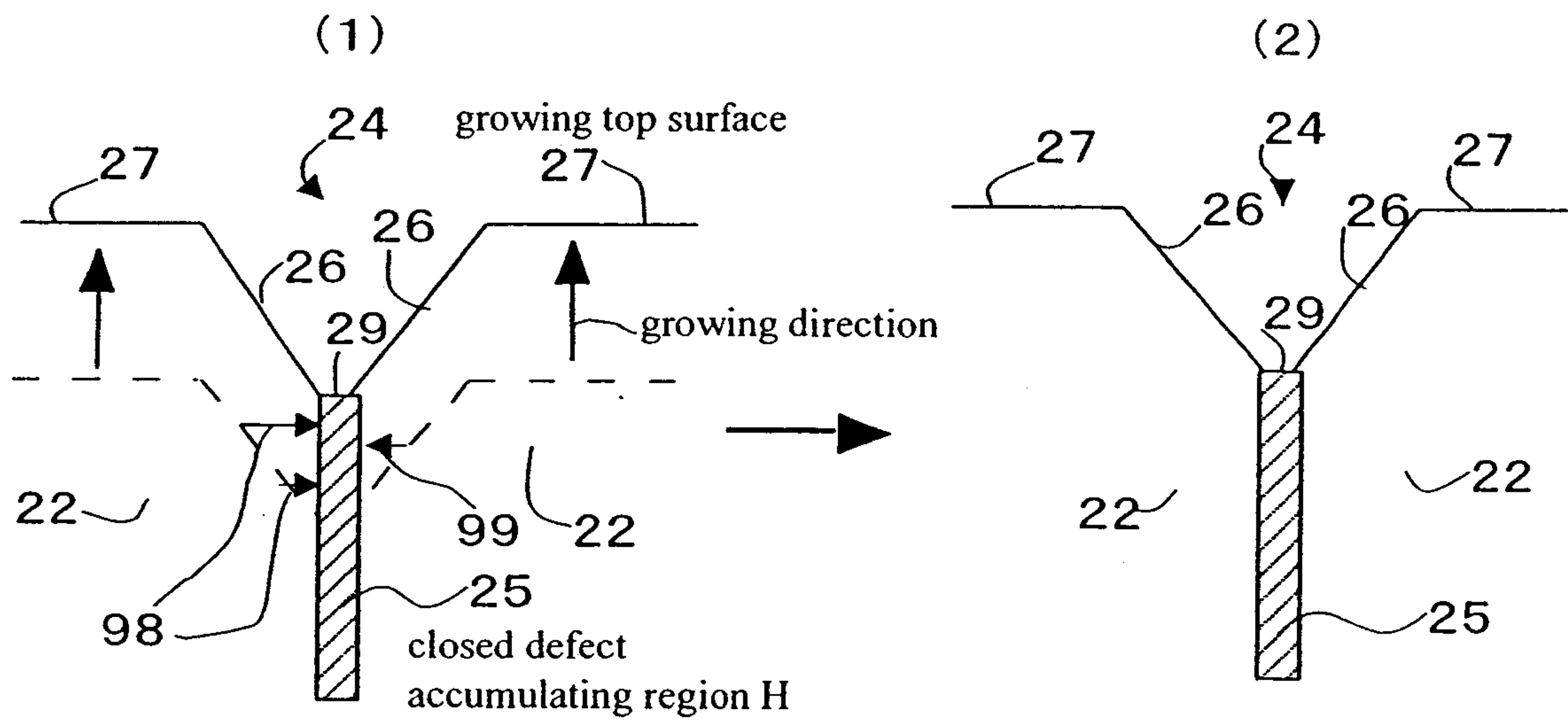
Fig.4 growing method of the present invention
