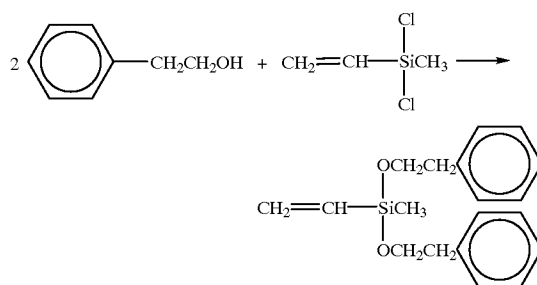
Reaction scheme II:
