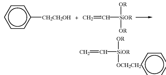
Reaction scheme III:
