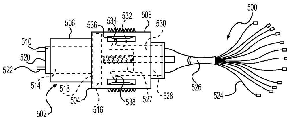
FIG. 5 (Conventional Art)
